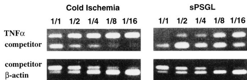
Figure 3. Examples of semiquantification by competitive RT-PCR assay. TNF \alpha mRNA expression in a cold ischemic kidney and in a kidney at 3 d after sPSGL treatment is compared. Expression of TNF \alpha and \beta -actin control mRNA were quantitated by the amount of competitive template that most nearly equaled the amplification of cellular cDNA. Compared to \beta -actin expression (equivalent point is 1/2), TNF \alpha expression of cold ischemia is 2.0 (equivalent point is 1/1), and that of sPSGL-treated animal is 0.25 (equivalent point is 1/8) in this sample.
