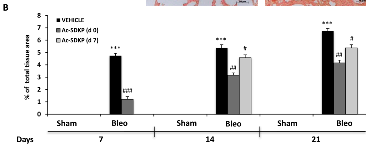
Figure 7: Ac-SDKP treatment inhibited BLEO-induced TGF- \beta expression in mouse lung tissue. (A) Representative microphotographs of TGF- \beta IHC in FFPE lung tissue slices from the indicated mice/groups/time points by using an anti-mouse TGF- \beta rabbit polyclonal antibody. (B) Densitometric analysis of the microphotographs using Optilab Graftek software: positive areas are expressed as percentage of total tissue area. The asterisks indicate a P < 0.05 versus Sham, ### P < 0.05 versus Bleomycin.
