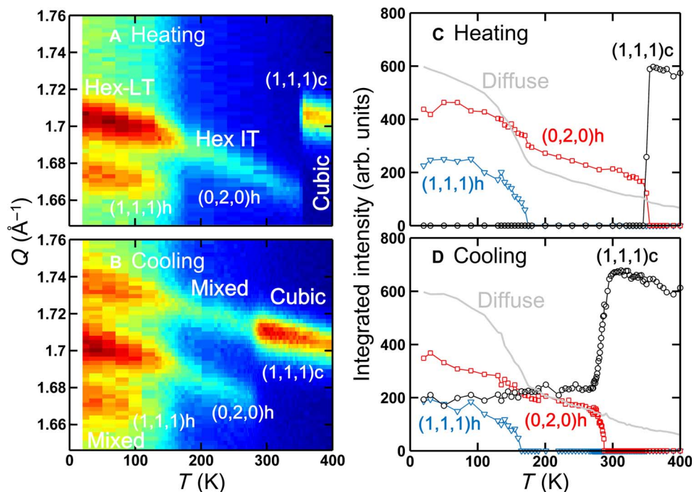
Fig. 2. Structural thermal hysteresis. Elastic neutron scattering data obtained from \text{FAPbI}_3 at SPINS, NCMR, upon heating (A and C) and upon cooling (B and D). (A) and (B) are contour maps of the scattering intensity as a function of momentum transfer, Q , and temperature, T . Q range of 1.65 to 1.76 \text{\AA}^{-1} was covered to probe the distinctive nuclear Bragg peaks— (1,1,1)_c , (0,2,0)_h , and (1,1,1)_h —associated with the cubic, Hex-IT, and Hex-LT phases, respectively. (C) and (D) are integrated intensities of the three peaks— (1,1,1)_c (black circle), (0,2,0)_h (red square), and (1,1,1)_h (blue triangle)—as a function of temperature. The light gray line indicates the temperature-dependent diffuse scattering intensity, as explained in the text.
