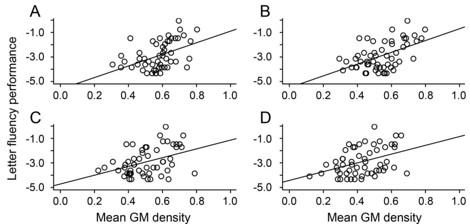
Figure 2 Higher gray matter density (GMD) associated with higher cognitive reserve (CR) and superior letter fluency
