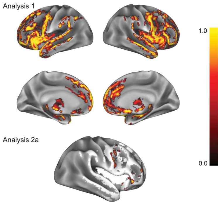
Analysis 1: Results of a nonparametric t test show regions of reduced GMD in patients with FTLD ( n = 55 ) relative to demographically comparable controls ( n = 90 ). Analysis 2a: Results of a regression analysis in patients with FTLD ( n = 55 ) restricted to regions of reduced GMD from analysis 1 (white regions) demonstrate that higher GMD in the right dorsolateral prefrontal cortex, rostral frontal cortex, orbital frontal cortex, and inferior frontal gyrus is associated with higher CR index. Color bar represents 1 - p value with yellow representing highest significance.
