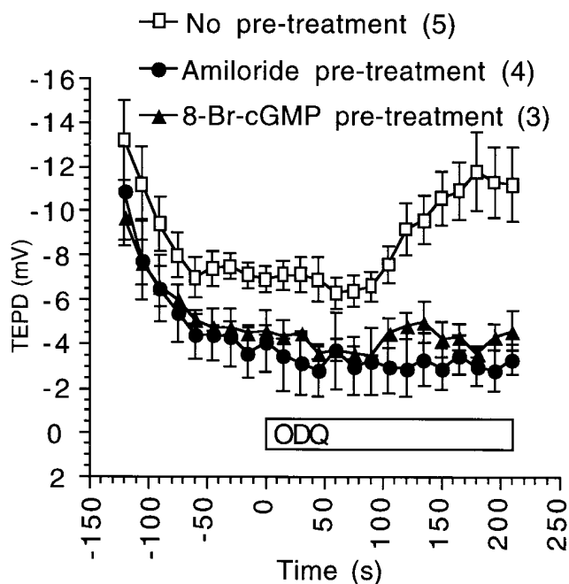
Figure 6. The effects of GC-S inhibition on mouse nasal TEPD in cfr (+/+, -) mice. The effect of the GC-S inhibitor ODQ (100 \mu M) on mouse nasal TEPD without pretreatment ( \square ) or in the presence of either amiloride (100 \mu M) ( \bullet ) or 8-Br-cGMP (100 \mu M) ( \blacktriangle ). The presence of ODQ is shown by the open bar. Number of experiments for each group is given in parentheses. Error bars represent SEM.
