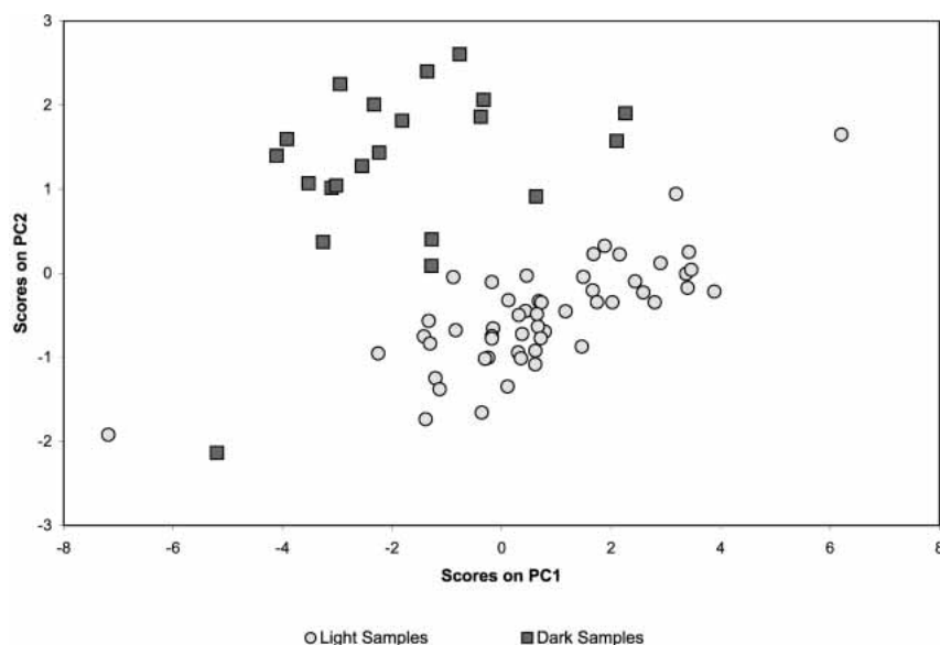
Figure 5 Two-dimensional mean-centered Principle Components Analysis of all 74 time points, using only the 113 genes.
