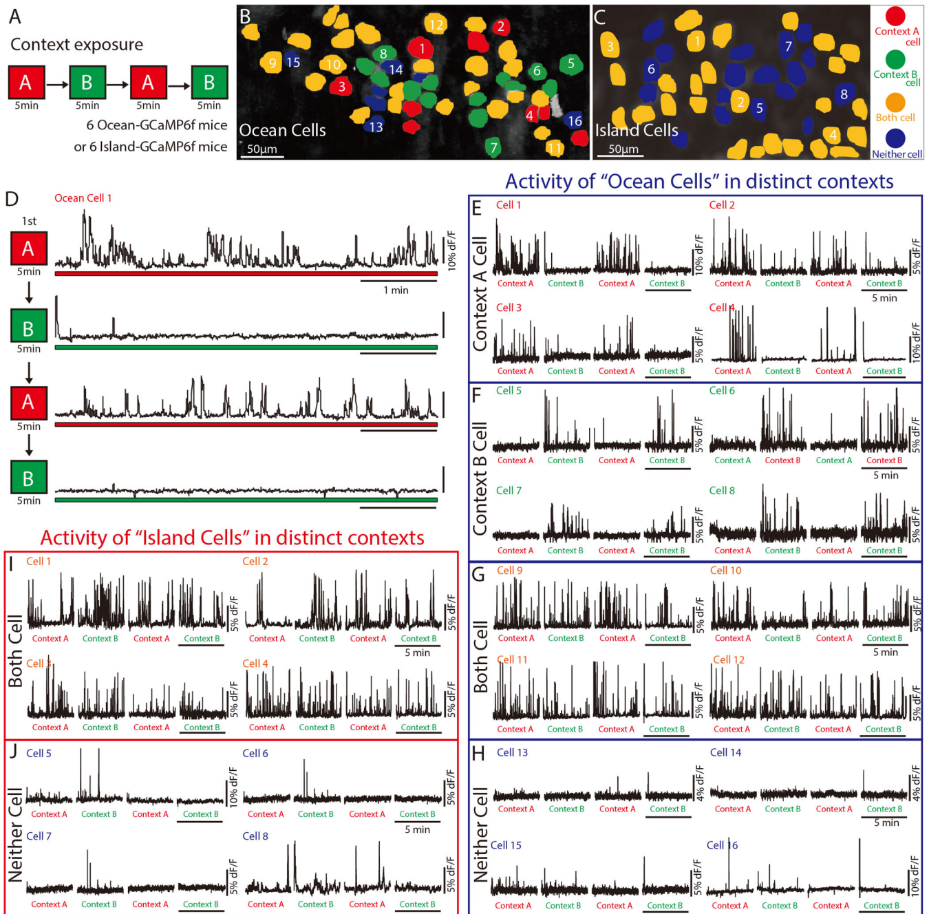
Fig. 2. Ocean cells, but not Island cells, exhibit context-specific \text{Ca}^{2+} activity
