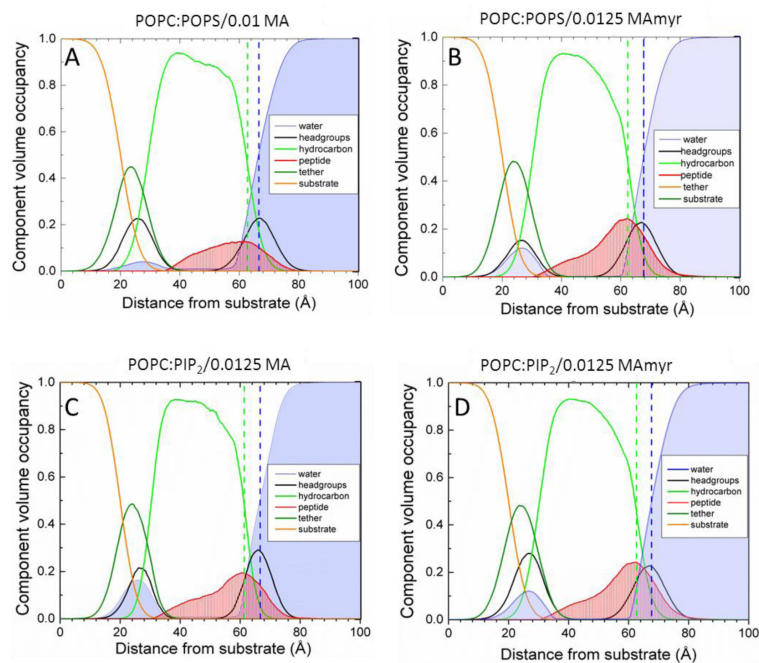
Figure 9. Scattering density profiles obtained from neutron reflectivity. A. POPC/POPS (60:40 mole ratio)/0.01 MA 31 , B. POPC/POPS (60:40)/0.0125 MA 31 myr, C. POPC/PIP 2 (90:10)/0.0125 MA 31 , D. POPC/PIP 2 (90:10)/0.0125 MA 31 myr. Bilayer components are shown in the legends; Gibbs dividing surfaces HC (green dashed line) and water (blue dashed line) are shown.
