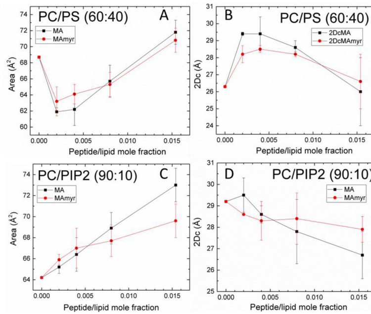
Figure 6. Structural results vs. increasing peptide mole ratio: (A) area/lipid A_L in POPC/POPS (60:40), (B) hydrocarbon thickness 2D_C in POPC/POPS (60:40), (C) A_L in POPC/PIP 2 (90:10), (D) 2D_C in POPC/PIP 2 (90:10). Error bars indicate the standard deviations of the average of 2-5 fits.
