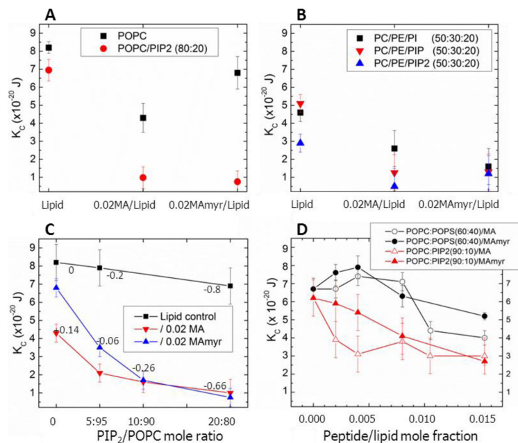
Figure 3. Bending modulus, K_C , as a function of lipid and peptide concentration. (A) 0.02 MA 31 or MA 31 myr in POPC, in POPC/PIP 2 (80:20), (B) 0.02 MA 31 and MA 31 myr in POPC/POPE/PI (50:30:20), in POPC/POPE/PIP (50:30:20), in POPC/POPE/PIP 2 (50:30:20), (C) 0.02 MA 31 or MA 31 myr in POPC with increasing PIP 2 , (D) Increasing MA 31 or MA 31 myr in POPC/pOpS (60:40) or POPC/PIP 2 (90:10). Numbers in Figs. 3C indicate the net membrane charge/lipid plus protein. Lipid control indicates samples with no peptides. Error bars represent standard deviations of the average K_C values from 2-5 different samples.
