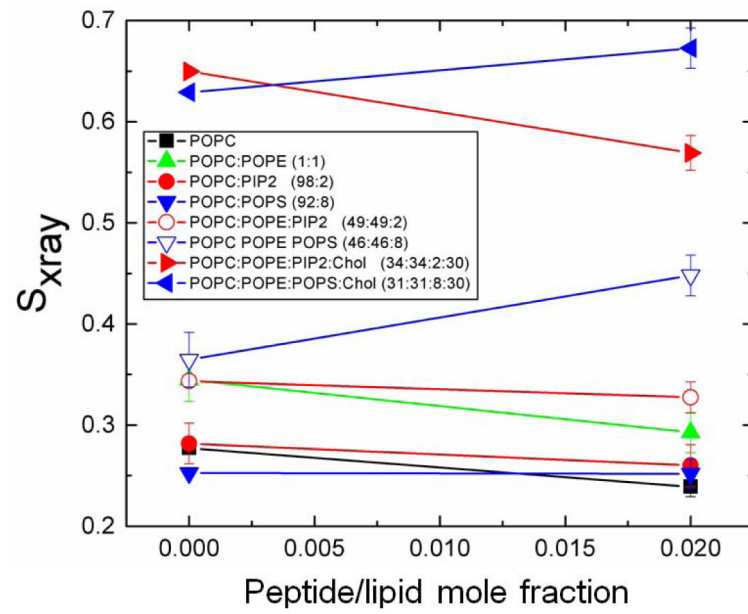
Figure 8. S_{xray} order parameter for pure lipid mimetics and MA 31 myr (see legend for lipid details). S_{xray} values were corrected for mosaic spread. Error bars represent standard deviation of average S_{xray} values from 2-4 images.
