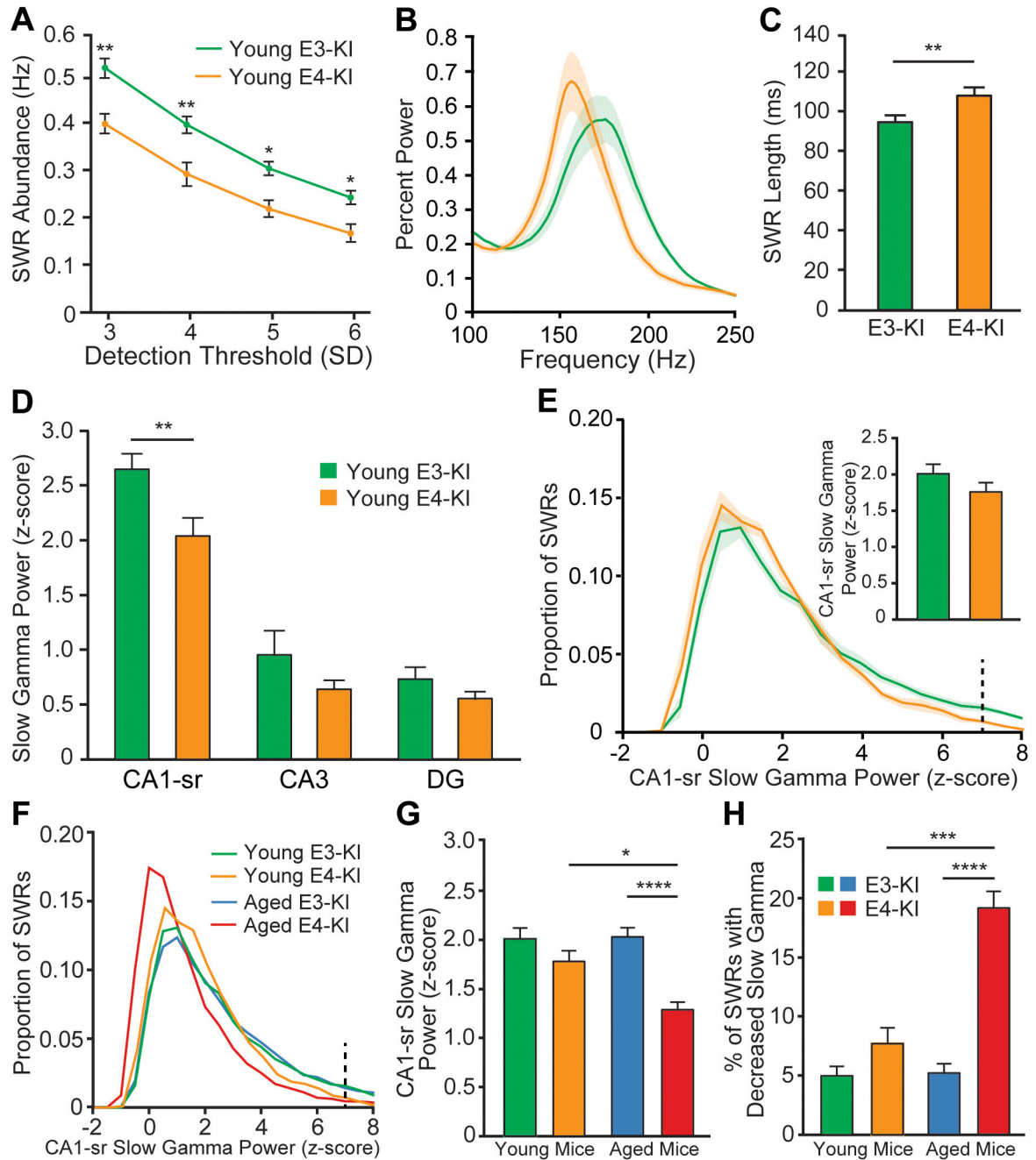
Figure 6. SWR and SWR-associated slow gamma characteristics in young apoE3-KI and apoE4-KI mice are differentially affected by aging
