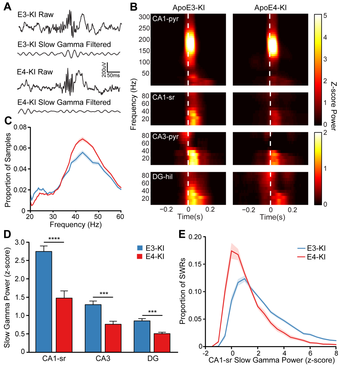
Figure 4. SWR-associated slow gamma power is reduced in aged apoE4-KI mice
