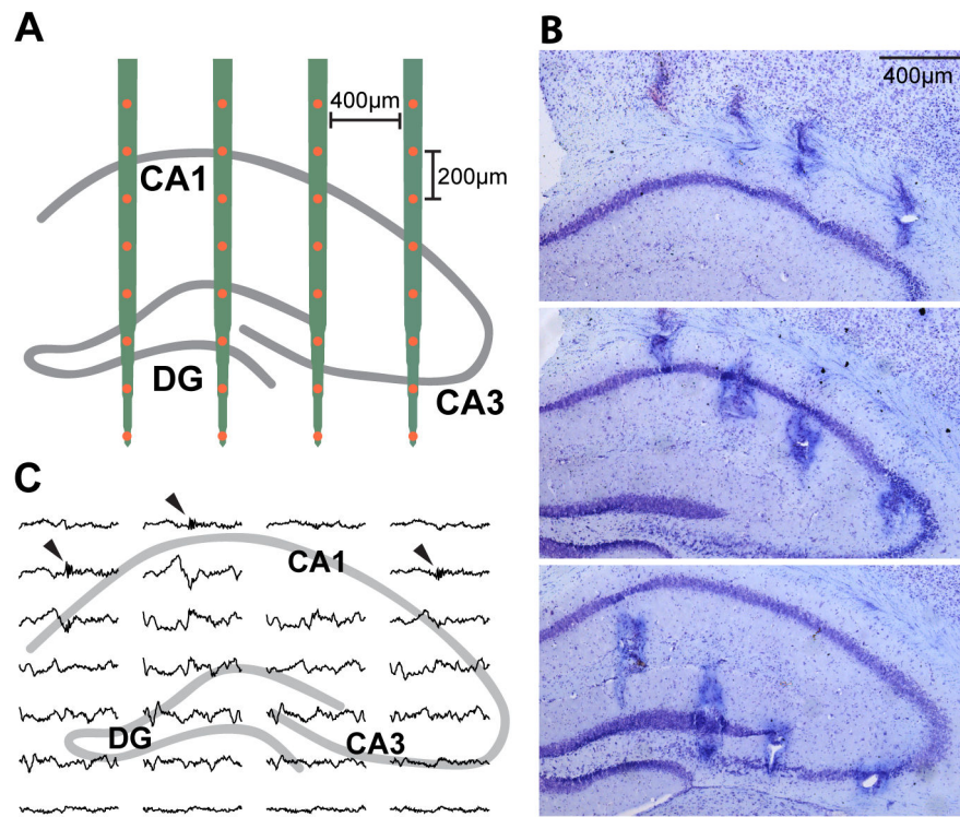
Figure 1. LFP recording of hippocampal network activity in apoE3-KI and apoE4-KI mice (A) Schematic representation of probe placement in the dorsal hippocampus, targeting CA1, CA3, and the DG. (B) Representative Nissl staining of brain sections after electrolytic lesioning indicates probe placement, shown in sequential coronal sections. (C) Sample data (800 ms) shown across all recording sites. Arrowheads indicate SWRs in CA1 pyramidal cell layer sites.
