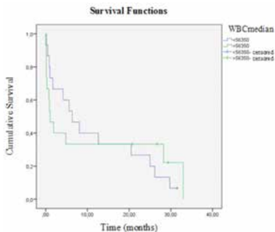
Figure 6. Kaplan-Meier curves of acute myeloid leukemia patients according to white blood cell count. WBC: White blood cell.
