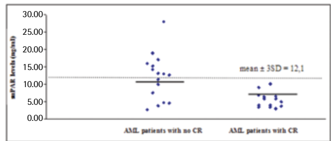
Figure 3. Soluble urokinase plasminogen activator receptor concentrations in serum from acute myeloid leukemia patients with no complete remission and acute myeloid leukemia patients with complete remission. The dotted line indicates the mean value plus 3 standard deviations of serum of acute myeloid leukemia patients with complete remission (12.1 ng/mL). suPAR: Soluble urokinase plasminogen activator receptor, AML: acute myeloid leukemia, SD: standard deviation, CR: complete remission.
