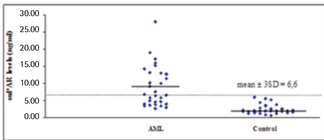
Figure 1. Soluble urokinase plasminogen activator receptor concentrations in serum from acute myeloid leukemia patients and healthy controls. The dotted line indicates the mean value plus 3 standard deviations of healthy control serum (6.6 ng/mL). suPAR: Soluble urokinase plasminogen activator receptor, AML: acute myeloid leukemia, SD: standard deviation.
