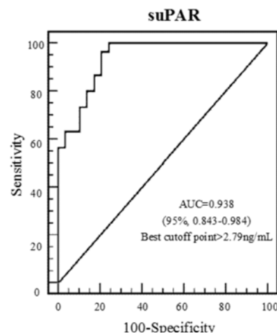
Figure 4. The receiver operating characteristic curves of acute myeloid leukemia patients according to soluble urokinase plasminogen activator receptor levels. suPAR: Soluble urokinase plasminogen activator receptor, AUC: area under the curve.
