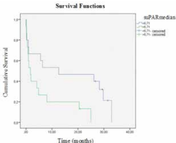
Figure 5. Kaplan-Meier curves of acute myeloid leukemia patients according to soluble urokinase plasminogen activator receptor levels. suPAR: Soluble urokinase plasminogen activator receptor.
