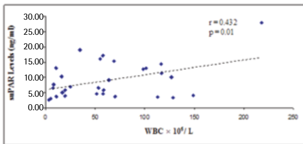
Figure 2. Correlations between soluble urokinase plasminogen activator receptor levels and white blood cell count in acute myeloid leukemia patients. WBC: White blood cell, suPAR: soluble urokinase plasminogen activator receptor, AML: acute myeloid leukemia.
