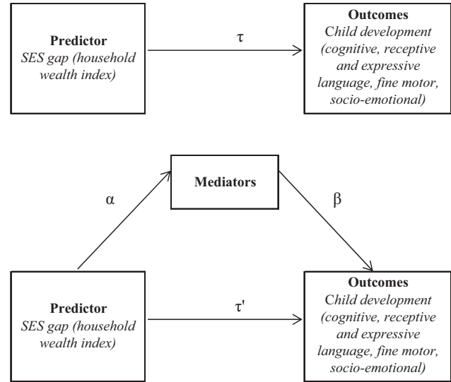
Figure 1. Mediation Model.
