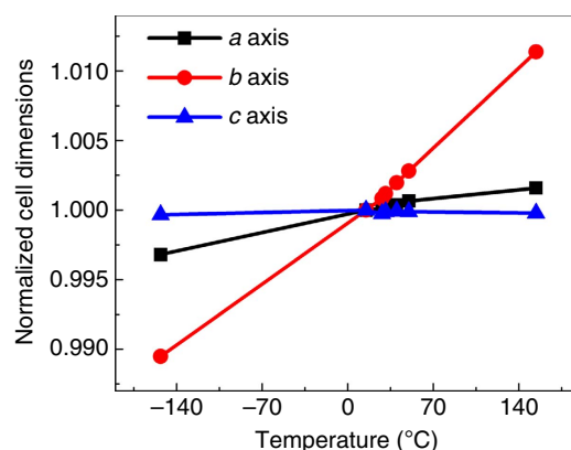
Figure 3 | Temperature variation of \alpha -glycine cell parameters. The values are normalized with respect to those at 15 °C (figure is constructed from the data taken from ref. 22). The b axis strongly increases with temperature, a far greater change than the changes in the other lattice parameters.
