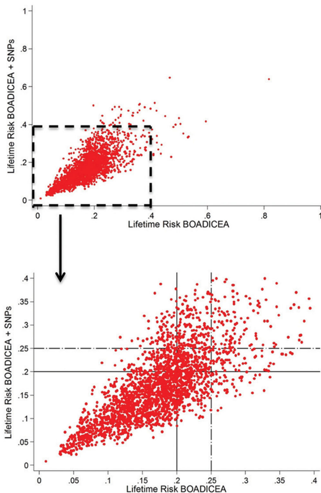
Figure 2. Scatter plot of BOADICEA lifetime risk against estimated lifetime risk based on the combination of BOADICEA score and the individual PRS. In the bottom panel solid horizontal and vertical line indicate the 20% threshold of lifetime risk while dashed lines denote the 25% threshold. Each red dot corresponds to an individual woman in the prospective cohort. Those in the upper left and lower right quadrants would be those who potentially could have a change in screening recommendations based on current guidelines.
