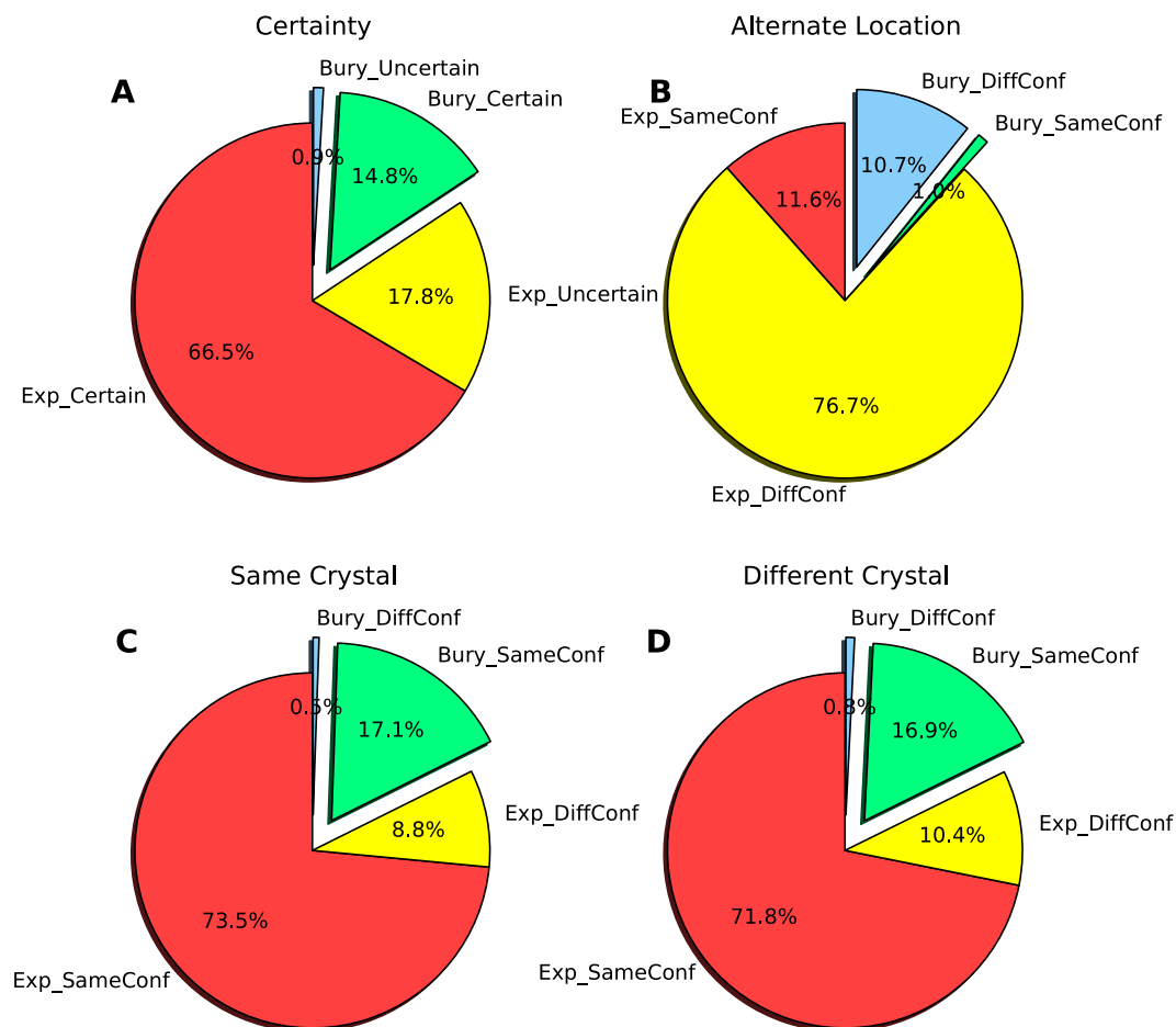
Figure 3. Pie plots of residue exposure and conformational variations, derived from dataset set1.
