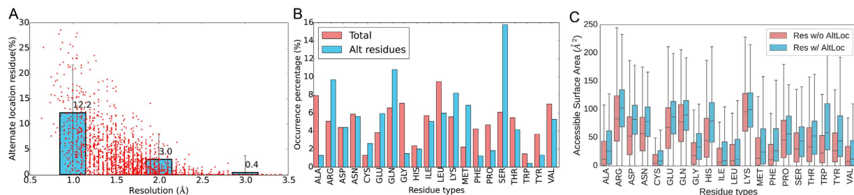
Figure 4. Alternate location counts, derived from dataset set1. (A) Percentages of alternate location residues. Each protein in the data set is presented as a red dot. X-axis is the resolution while y-axis is the percentage of residue counted in a protein. The blue histograms show the average percents of alternate location residues in proteins <1.0\text{ \AA} , 1.0\text{--}2.0\text{ \AA} and 2.0\text{--}3.0\text{ \AA} resolution. Error bars show the standard deviations. (B) Residue type occurrences. Occurrence of each residue type was counted for all residues and for alternate location residues. Arg, Glu, Gln, Lys, Met and Ser show more occurrences in alternate location residues. (C) Average residue accessible surface area (RSA) of residues with and without alternate location atoms. Red box plots 'Res w/o AltLoc' show the RSA distribution of residues without alternate location atoms, while blue box plots show the RSA distribution of residues with alternate location atoms.
