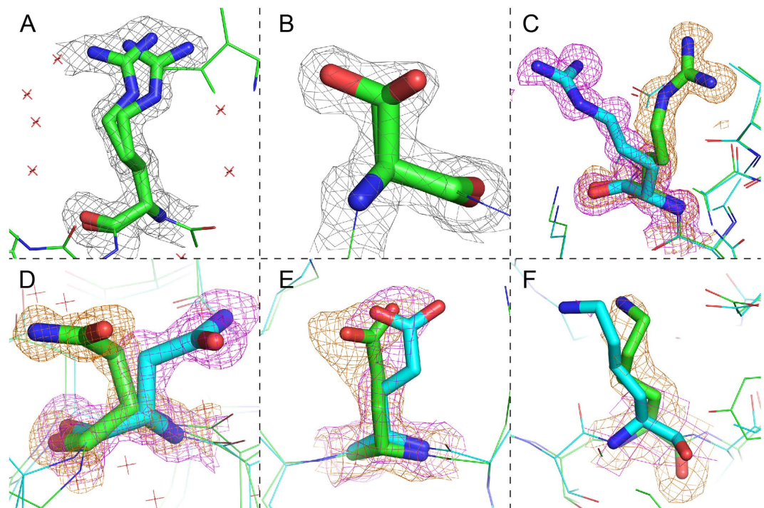
Figure 1. Side-chain conformational variation examples. (A) Arg6 in plv4264 protein (4mv2) structure has two alternate locations, resolution 1.35 Å. State A has 0.45 occupancy, while state B has 0.55 occupancy. (B) Ser141 in 4b1y chain B includes two discrete alternate locations of 0.66 and 0.33 occupancies. (C) Arg112 in lysozyme C protein (3wl2, resolution 0.96 Å) chain A (green) and B (blue). Sequence identity of the two chains is 100%, while TMscore is >0.98. Electron density in both the structures are clear, while occupancies of all the atoms equal to 1. (D) Asn44 in 2vb1 (green, in chain A, resolution 0.65 Å) and 1iee (cyan, in chain A, resolution 0.94 Å). Both the chains are lysozyme C protein structures in Gallus gallus sharing 100% sequence identity and 0.97 TMscore, solved by different labs. Electron density map of 2vb1 is shown in green and 1iee is shown in blue. Both the residues have clear electron density for all the atoms. (E) Glu81 in 4pj2 (green, in chain A, resolution 1.24 Å) and 3od9 (cyan, in chain A, resolution 1.41 Å). Both the chains are periplasmic lysozyme inhibitor of I-type lysozyme structures in Aeromonas hydrophila sharing 100% sequence identity and >0.97 TMscore, solved by the same lab. Electron density map of 4pj2 is shown in green and 3od9 is shown in blue. The residue of 4pj2 has clear electron density for all the atoms, while not all of the atoms have clear electron density in 3od9. (F) Lys95 in 2pa8 (green, in chain D, resolution 1.76 Å) and 2pmz (cyan, in chain (D), resolution 3.4 Å). Both the chains are DNA-directed RNA polymerase subunit D structures in Sulfolobus solfataricus sharing 100% sequence identity and >0.91 TMscore, solved by the same lab. Electron density map of 2pa8 is shown in green and 2pmz is shown in blue. The residue of 2pa8 has clear electron density for all the atoms, while none of the side-chain atoms has clear electron density.
