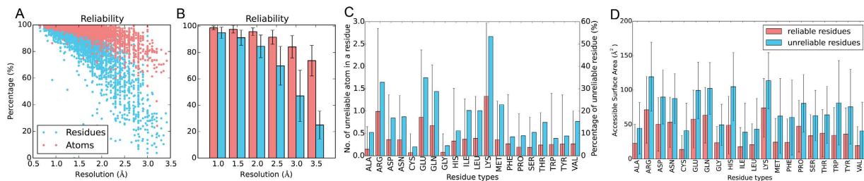
Figure 2. Atom reliability based on electron density, derived from dataset set I. (A) Percentage of reliable atoms/residues in PDB structures. X-axis is the resolution of the PDB structures, while y-axis is the percentage of the reliable atoms/residues. The percentage of reliable atoms (electron density >1\sigma , only atoms from the first conformer is considered) is shown as a red dot for each protein, while the percentage of reliable residues (all atoms are reliable) is shown as a blue dot. (B) Average percentage of reliable atoms/residues in PDB structures. X-axis is the resolution of the PDB structures. The bars are the averaged percentages and error bars show the standard deviations. (C) Average percentage of reliable atoms/residues counted by residue types. Average number of atom with low electron density ( \sigma < 1 ) are shown in red on left y-axis and percentages of unreliable residue (residue include more than one low electron density atom) are shown in blue right y-axis. (D) Histogram comparison between average residue accessible surface area of reliable and unreliable residues.
