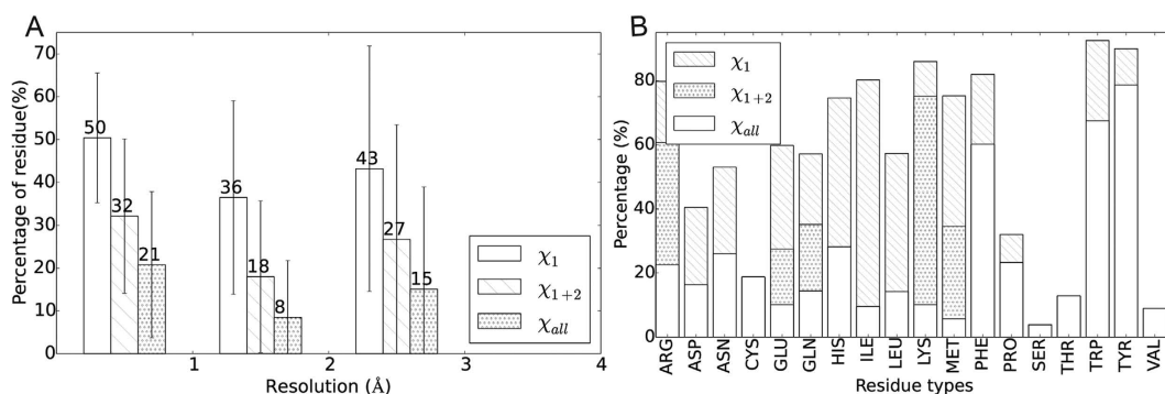
Figure 5. Conformational variation rate of alternate location residues, derived from dataset set1. (A) Percentage of alternate location residue that keep the same conformation in different conformational states counted by protein. Average values are counted for proteins <1.0\text{ \AA} , 1.0\text{--}2.0\text{ \AA} and 2.0\text{--}3.0\text{ \AA} resolution and shown as histograms, where error bars show the standard deviations. \chi_1 , \chi_{1+2} and \chi_{all} mean the \chi dihedral angles that are kept the same in the residue. (B) Percentage of alternate location residue that keep the same conformation in different conformational states counted by residue types.
