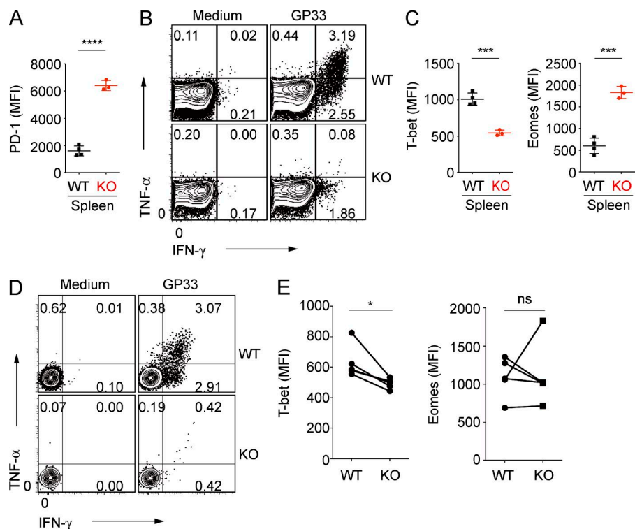
Figure 5. TMEM16F regulates T cell response in a cell-intrinsic manner. (A–C) WT or TMEM16F-deficient BM chimeric mice were i.v. infected with 4 \times 10^5 pfu LCMV clone 13 and sacrificed at day 150 after infection. Expression of PD-1 (A) and T-bet and Eomes (C) in GP33-tetramer-positive CD8 T cells, and cytokine production in CD8 T cells after stimulation with GP33 (B) were analyzed by flow cytometry. n = 4 for WT; n = 3 for KO. (D and E) Mixed BM chimera were infected as in A–C. Mice were sacrificed at day 150 after infection. Cytokine production in WT or KO CD8 T cells after stimulation with GP33 in D, and expression of T-bet and Eomes in GP33-tetramer-positive CD8 T cells in E, were determined by flow cytometry. n = 4 for each group. MFI, mean fluorescence intensity. Results are displayed as mean \pm SEM of at least two independent experiments. *, P < 0.05 ; ***, P < 0.001 ; ****, P < 0.0001 ; ns, not significant, using Student's t test.
