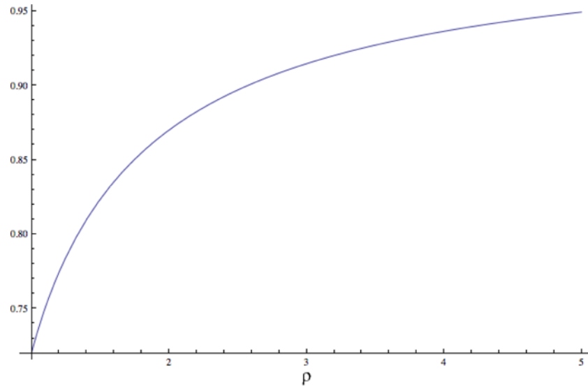
Figure 2. Plot of \varepsilon(\rho) = \lim_{d \rightarrow \infty} a_{\mathbb{R}}(d, \rho d) for \rho \in [1, 5] .
