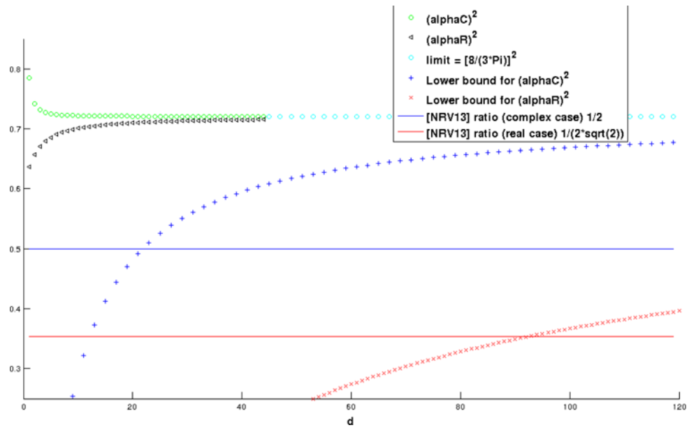
Figure 1. Plot showing the computed values of \alpha_{\mathbb{K}}(d)^2 , for d \leq 44 , the limit of \alpha_{\mathbb{K}}(d)^2 as d \rightarrow \infty , the lower bound for \alpha_{\mathbb{K}}(d)^2 given by Theorem 7 as function of d , and the approximation ratio of \frac{1}{2\sqrt{2}} and \frac{1}{2} obtained in [NRV13].
