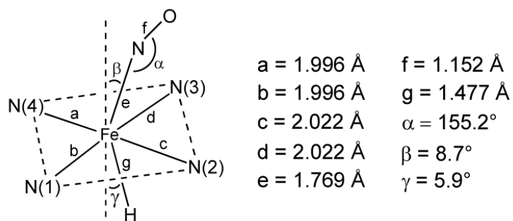
Fig. 6. Selected geometrical parameters (in \text{\AA} and degrees) for DFT-calculated (OEP)Fe(NO)H. The tilting angles are with respect to the four-nitrogen porphyrin plane.
