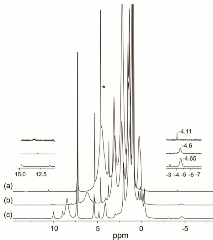
Fig. 5. 1 H NMR spectra (in CDCl 3 ) of the reaction to generate (OEP)Fe(NO)H, highlighting the upfield and downfield regions of (a) (OEP)Fe(NO)H (top spectrum), (b) (OEP)Fe(H) byproduct (middle spectrum), and (c) (OEP)Fe(H) from the control reaction of [(OEP)Fe]OTf with hydride (bottom spectrum). The peak labeled * is due to the H 2 decomposition product (see text).
