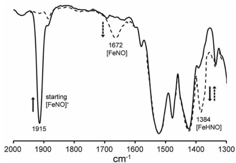
Fig. 2. IR spectroscopic characterization of the bound HNO ligand in (\text{PPDME})\text{Fe}(\text{HNO})(1\text{-MeIm}) , showing formation of the \nu_{\text{NO}} 1384 \text{cm}^{-1} band (dashed line) upon hydride addition to the cationic precursor ( \nu_{\text{NO}} 1915 \text{cm}^{-1} ). The new 1384 \text{cm}^{-1} band slowly converts to the band at 1672 \text{cm}^{-1} .
