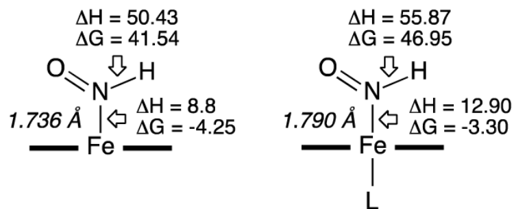
Fig. 8. Bond strength energies ( \Delta H and \Delta G ) for the five-coordinate and six-coordinate Fe-HNO systems (L = 5-MeIm). Values are in kcal/mol.
