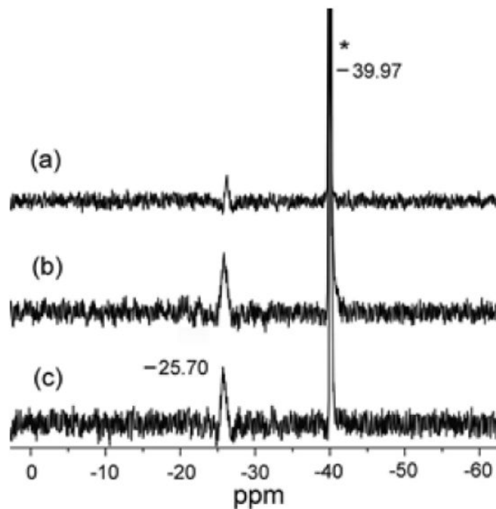
Fig. 7. ^{11}\text{B}\{^1\text{H}\} NMR spectra of the product mixtures from (a) the reaction of [(\text{OEP})\text{Fe}(\text{NO})(5\text{-MeIm})]\text{OTf} with excess [\text{NBu}_4]\text{BH}_4 (signal at -40 ppm), and (b) the reaction of [(\text{OEP})\text{Fe}(\text{NO})]\text{OTf} with excess [\text{NBu}_4]\text{BH}_4 , and (c) the control and known reaction of [\text{NBu}_4]\text{BH}_4 with 1,2-dichloroethane to generate diborane. 25
