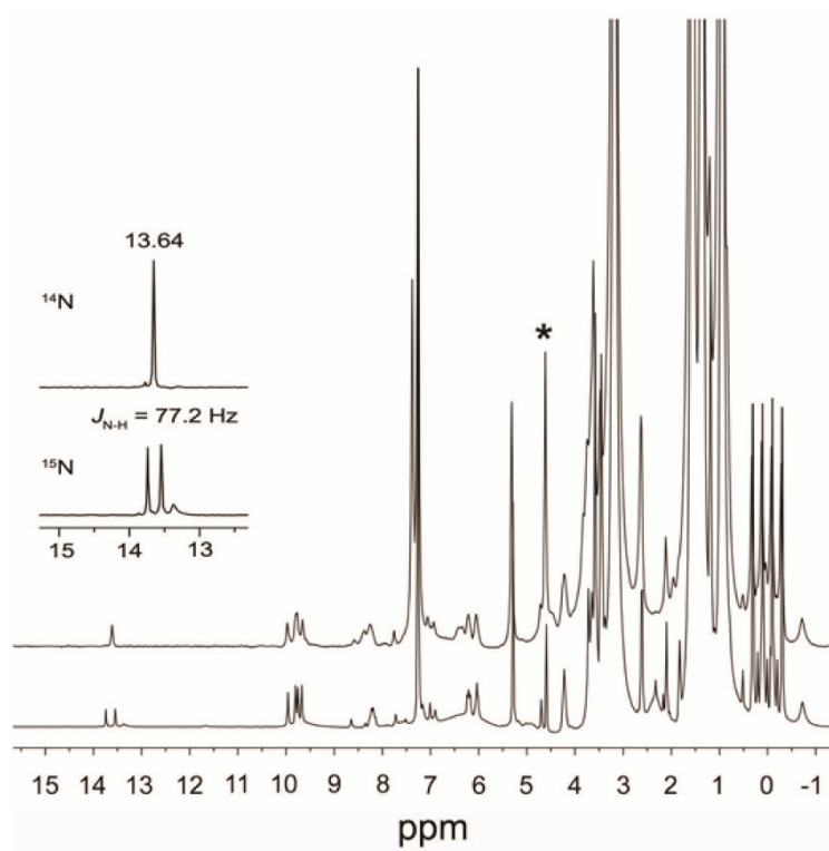
Fig. 3. ^1\text{H} NMR spectra (in \text{CDCl}_3 ) of the reaction of [(\text{PPDME})\text{Fe}(\text{NO})(1\text{-MeIm})]\text{OTf} with [\text{NBu}_4]\text{BH}_4 to generate (\text{PPDME})\text{Fe}(\text{HNO})(1\text{-MeIm}) . The bottom spectrum showing the splitting of the Fe-HNO peak at 13.64 ppm into a doublet was obtained using [(\text{PPDME})\text{Fe}(^{15}\text{NO})(1\text{-MeIm})]\text{OTf} in the reaction. The peak labeled * is due to the \text{H}_2 decomposition product (see text and Fig. S2).
