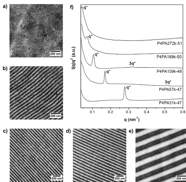
Figure 1. a)–e) Bright-field TEM images of iodine-stained P4PA diblock copolymers. P4VP appears dark. P4PA31k-47 (a), P4PA57k-47 (b), P4PA109k-48 (c), P4PA189k-50 (d), and P4PA272k-51 (e). f) Room-temperature Lorentz-corrected SAXS patterns of neat P4PA diblock copolymers.
