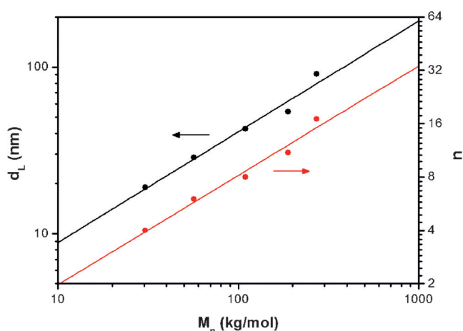
Figure 4. Molecular weights of P4PA in P4PA(3-NDP) 0.5 double-combs plotted against the large length scale d_L at T \approx 60^\circ\text{C} ( T > T_m ) and number of small repeating structures n ( = d_L/d_s ). Both parameters ( d_L and n ) scale as M_n^{0.67} .
