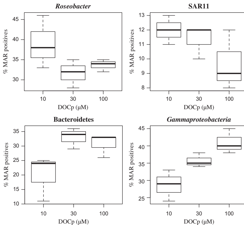
Figure 1 Box plots presenting the percentage of MAR-FISH-positive (cells actively taking up the radiolabeled compounds) within each heterotrophic bacterial phylogenetic group ( \text{MAR}^+_{\text{g}}/\text{CARD-FISH}^+_{\text{g}} , see text), for the different DOCp concentrations (grouping the results by the three different algal treatments). The central full line indicates the median value, the boxes indicate the lower and upper quartiles, and vertical lines indicate the 10th and 90th percentiles. Note the different scales on the y axes.
