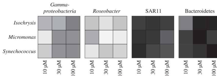
Figure 2 Bimodal heat map of the IS between marine heterotrophic bacteria phylogenetic groups and different DOC sources at different concentrations. Darker tones of gray indicate stronger IS (' \text{MAR}^+_{\text{g}} /DAPI counts' data from Table 1 and Figure 2). Roseobacter and SAR11 are both subgroups of Alphaproteobacteria .
