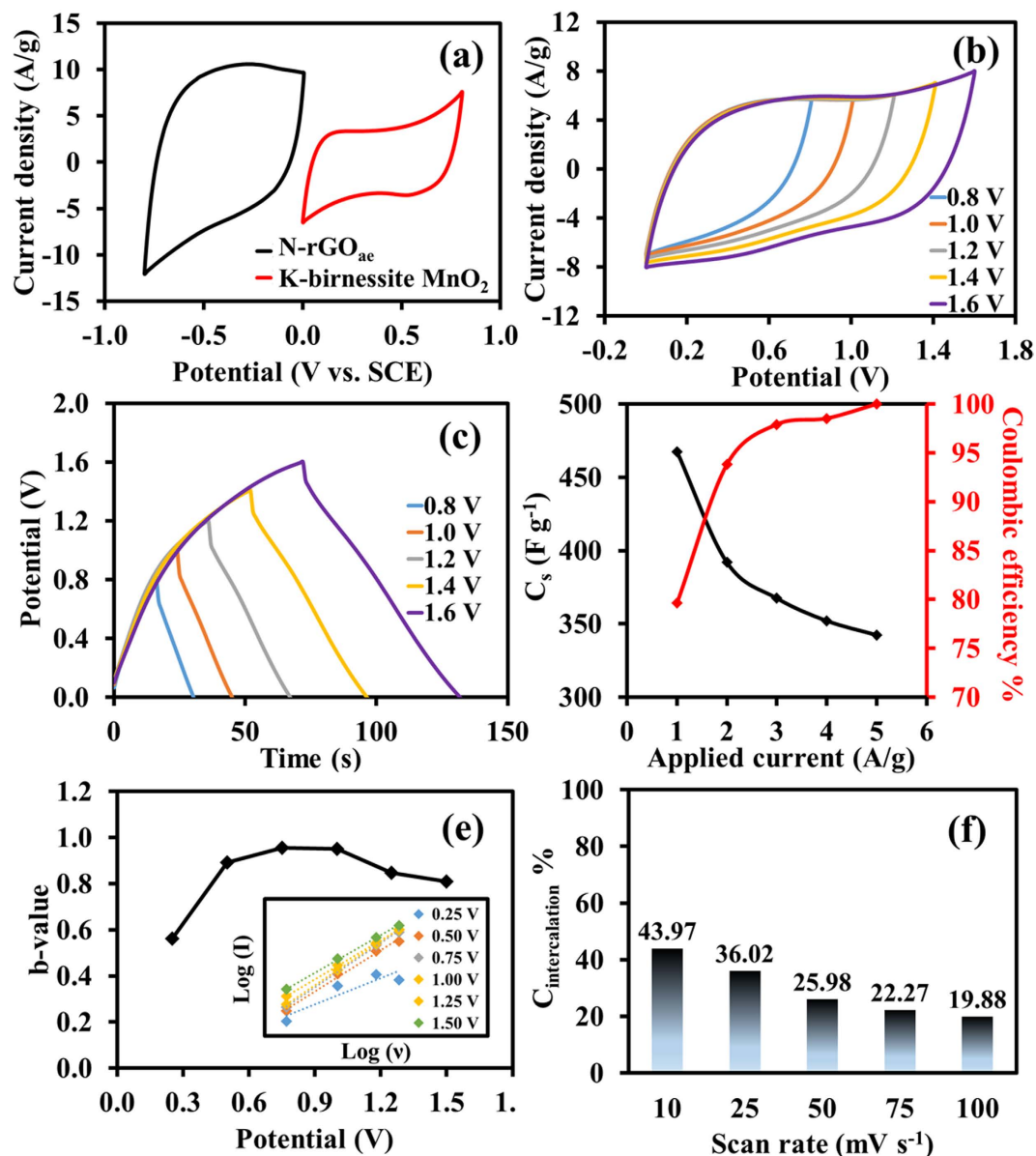
Figure 4. (a) CVs of the as-fabricated electrodes at 25 \text{ mV s}^{-1} and (b) CVs at different working potentials ( 50 \text{ mV s}^{-1} ), (c) GCDs at different working potentials ( 5 \text{ A g}^{-1} ), and (d) specific capacitance and coulombic efficiency vs. applied current density, (e) the b value as a function of potential, and (f) the bar chart of the diffusion-controlled intercalation capacitance vs. scan rates of as-fabricated MnO 2 //N-rGO ac supercapacitor devices.
