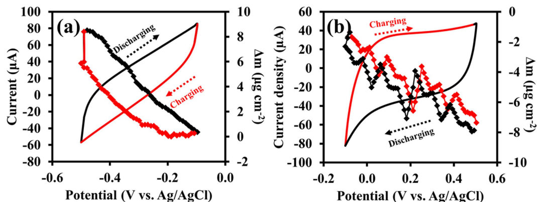
Figure 7. CVs at 25 \text{ mVs}^{-1} and in situ EQCM responses of (a) N-rGO ac and (b) MnO 2 electrodes.
