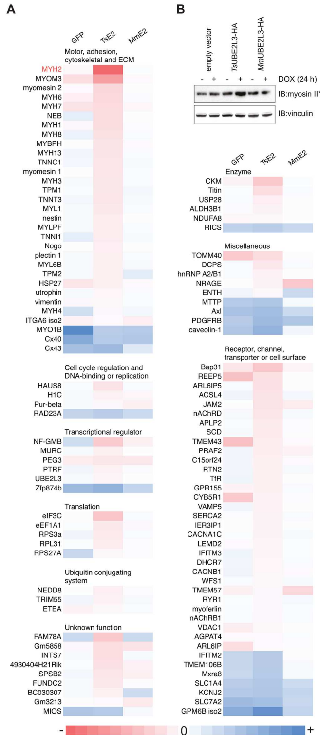
Fig 6. UbiScan analysis of TsUBE2L3 effect on the myotube ubiquitome. A. Heatmap displaying proteins in which ubiquitinated peptides were found to be upregulated (blue) or downregulated (red) as measured by a fold change in relation to the empty vector C2C12 myotube cell line after 24 h expression of eGFP-HA (GFP), TsUBE2L3 -HA (TsE2) or MmUBE2L3 -HA (MmE2). Proteins listed showed a maximum % CV of 49.9 or less, a maximum intensity of 200,000 or more and a fold change in ubiquitination of 2.5 or more in response to TsUBE2L3 -HA expression only. Where multiple ubiquitinated peptides were identified for the
