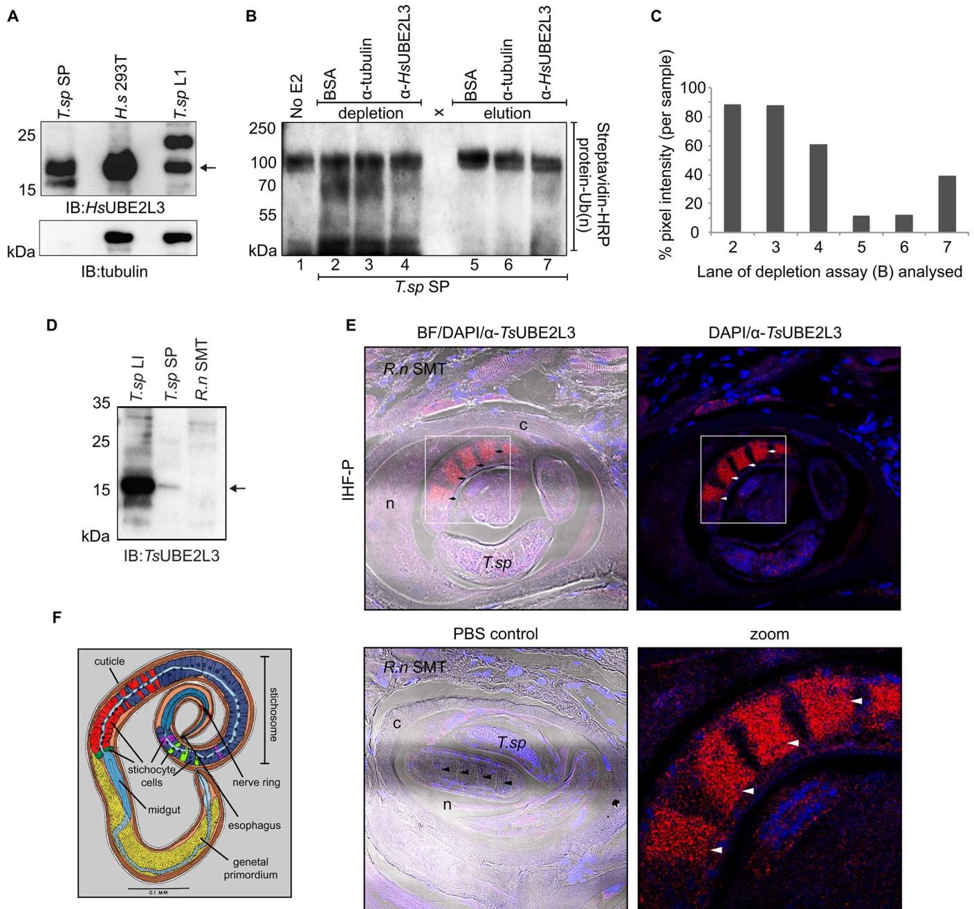
Fig 2. Verification of expression, secretion, activity and localization of TsUBE2L3. A. T.sp SP, HEK 293T cell lysate and T. spiralis muscle larvae lysate were separated by SDS-PAGE and immuno-blotted with anti- Hs UBE2L3 and anti-tubulin antibodies. B. Auto-ubiquitination of parkin with Ub-biotin was probed by streptavidin-HRP blot. Reactions from left to right: lane 1: human E1 (UBE1A), E3 (parkin) and Ub-biotin only (no E2). Reactions in lanes 2–4 included human E1, parkin and Ub-biotin, with the following E2 substitution: lane 2: T.sp SP after resin-bound BSA depletion (BSA), lane 3: T.sp SP after resin-bound anti-tubulin depletion ( \alpha -tubulin), lane 4: T.sp SP after resin-bound \alpha - Hs UBE2L3 depletion ( \alpha - Hs UBE2L3). In lanes 5–7 the elution fractions from the depletions shown in lanes 2–4 were used to substitute E2. C. The pixel intensity of lanes 2–7 of the depletion assay (B) was analysed using an ImageJ gel analysis plugin. For each of the three samples tested in the assay (BSA, \alpha -tubulin and \alpha - Hs UBE2L3) the sum of the pixel intensity of the depletion plus elution lanes was taken as 100% (intensity of lane 2 + 5 for BSA and so on). The relative percentages of the depletion and elution lanes were then calculated (intensity of lane 2/(2+5) x 100) and plotted. D. A Ts UBE2L3-specific antibody was made and its specificity was assessed by immuno-blot against T.sp L1 lysate, T.sp SP and rat ( R.n ) skeletal muscle tissue (SMT) lysate. The arrow indicates the expected size of Ts UBE2L3. E. T. spiralis infected rat skeletal muscle tissue ( R.n SMT) was sectioned and analyzed by immuno-histofluorescence. A single T.sp L1 inside the nurse cell (n), surrounded by a collagen capsule (c) is displayed. Tissue was probed with anti- Ts UBE2L3 antibodies (Alexa-568, red) and nuclei were stained using DAPI (blue). Brightfield (BF)/DAPI/anti- Ts UBE2L3 and DAPI/anti- Ts UBE2L3 merged images are displayed. As a control, infected R.n SMT was probed with PBS and DAPI only. Arrows indicate stacks of stichocyte cells in the stichosome. F. Annotated diagram of T. spiralis L1 morphology. Image adapted
