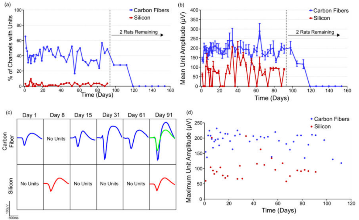
Figure 6. Chronic unit amplitudes and percentage of channels with units
