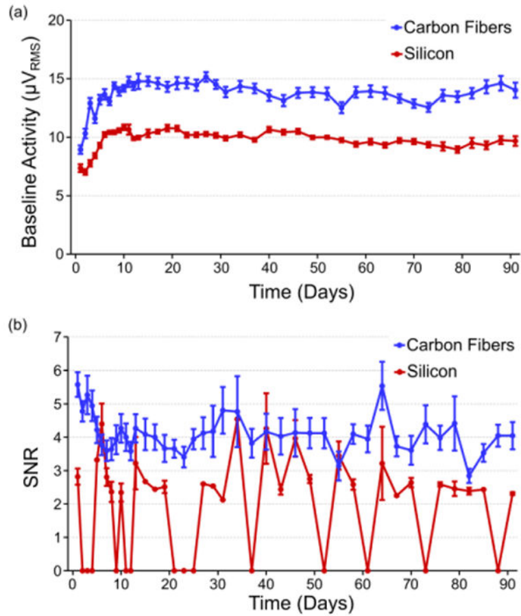
Figure 7. Chronic baseline activity and SNR
