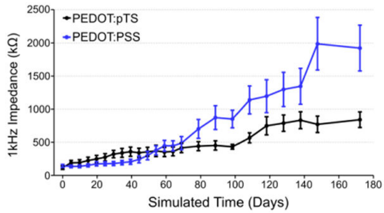
Figure 3. PEDOT soak test
