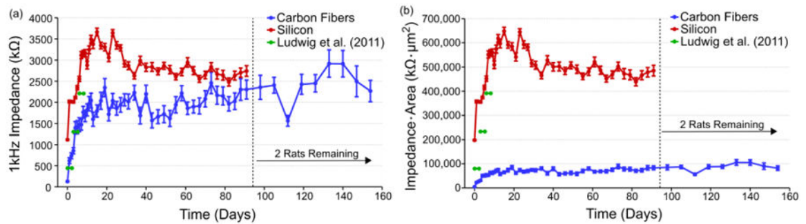
Figure 5. Chronic implant impedances
