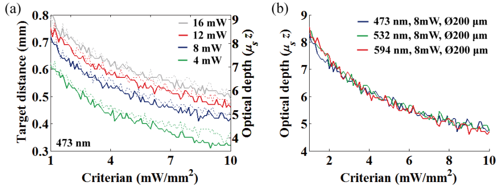
Fig. 6. Intensity criterion vs. OFD at 473 nm for the four different fiber output powers (4, 8, 12 and 16 mW). Dotted and thick solid lines represent 100 and 200 \mu\text{m} fiber diameters, respectively. (b) Intensity criterion vs. normalized OFD at the different wavelengths (473, 532, and 594 nm).
