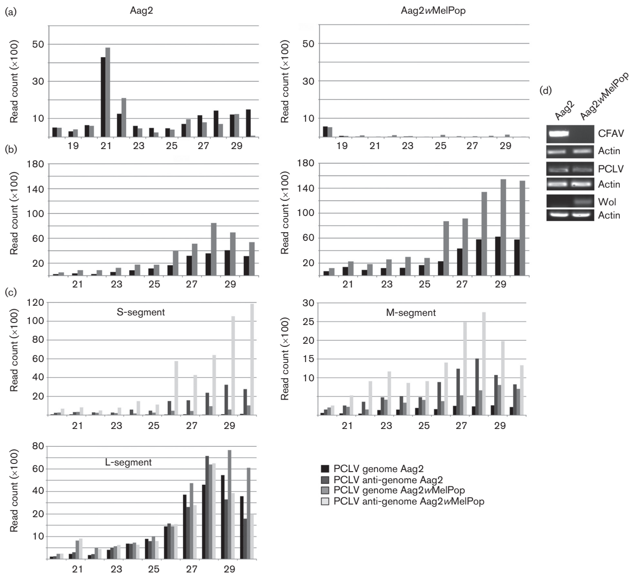
Fig. 1. Presence or absence of CFAV, PCLV and wMelPop in Aag2 and Aag2 wMelPop cells. Size distribution of small RNA molecules mapping to the CFAV (a) or PCLV (b) genome (black)/anti-genome (grey) in A. aegypti -derived Aag2 or wMelPop -transfected Aag2 cells. (c) Size distribution of small RNA molecules mapping to the different segments of PCLV (S, M and L) genome/anti-genome in A. aegypti -derived Aag2 or wMelPop -transfected Aag2 cells. (d) Detection of CFAV or PCLV in Aag2 and Aag2 wMelPop cells by RT-PCR. Actin was used as loading control.
