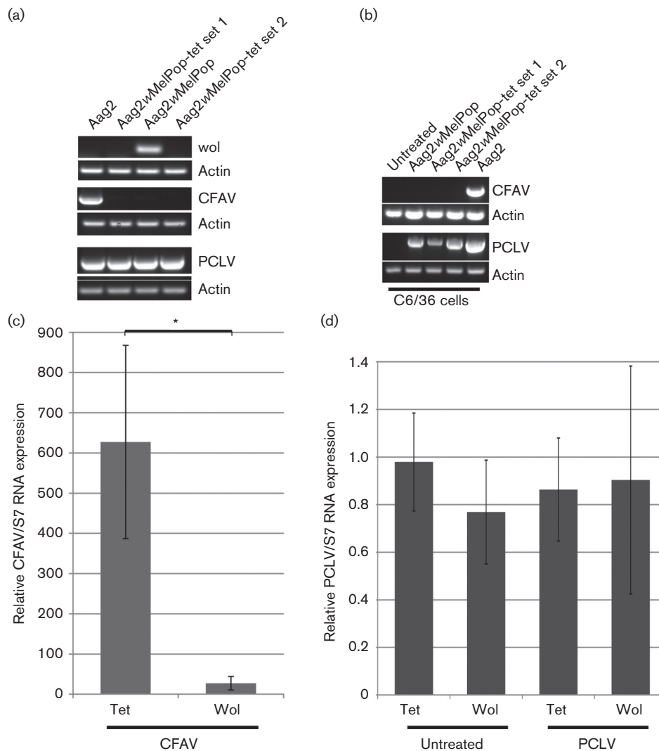
Fig. 2. Effect of wMelPop on CFAV and PCLV infection in Aag2 cells. (a) Detection of CFAV, Wolbachia or PCLV in Aag2, Aag2 wMelPop and two different cultures of Aag2 wMelPop -tet sets 1 and 2 cells by RT-PCR. Actin was used as loading control. (b) Detection of CFAV or PCLV in C6/36 cells incubated with supernatant of Aag2, Aag2 wMelPop or Aag2 wMelPop treated with tetracycline (two different cultures, Aag2 wMelPop -tet sets 1 and 2) by RT-PCR. Actin was used as a loading control. (c) Quantification of CFAV RNA in Aag2 wMelPop (Wol) or Aag2 wMelPop treated with tetracycline (Tet) cells after incubation with Aag2 supernatant containing CFAV by SYBR Green. S7 was used as internal control. Relative RNA expression is represented as (CFAV/S7). Error bars show SEM from three independent experiments. (d) Quantification of PCLV RNA in Aag2 wMelPop (Wol) or Aag2 wMelPop treated with tetracycline (Tet) cells, either after incubation with Aag2 supernatant harbouring PCLV or untreated by SYBR Green. S7 was used as an internal control. Relative RNA expression is represented as (PCLV/S7) and mock-infected tetracycline cells were set to 1. Error bars show SEM from three independent experiments. * P < 0.05 .
