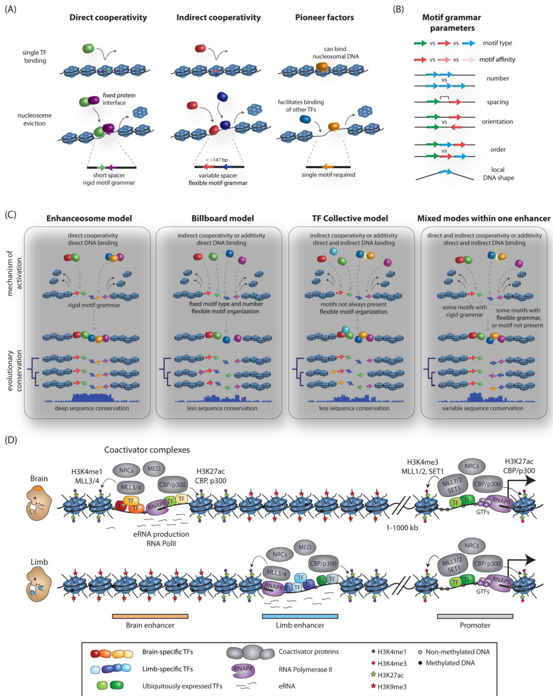
Figure 1. Nucleosome eviction, enhancer grammar and models of enhancer architecture (A) TF mechanisms for overcoming energetic barrier to nucleosomal eviction and underlying motif requirements. (B) Parameters of motif grammar at enhancers. (C) Models of enhancer architecture and their primary mechanism of TF binding, flexibility of motif organization, and selective constraint across evolution. (D) Coactivator binding and chromatin signatures at active enhancers. Presence of cell-type specific and broadly-expressed TFs, RNA Polymerase II (RNAPII) and associated enhancer RNAs (eRNAs), coactivator complexes such as Mediator (Med), nucleosome remodeling complexes (NRCs),
