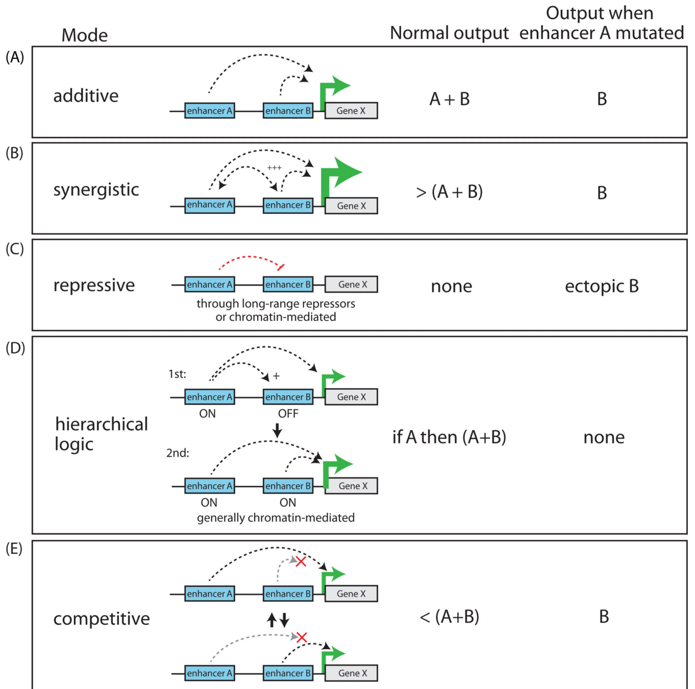
Figure 5. Regulatory crosstalk between enhancers operating within the same cis-regulatory landscape (A-E) Potential modes of enhancer relationships and their effect on transcriptional output under wildtype or mutant conditions.
