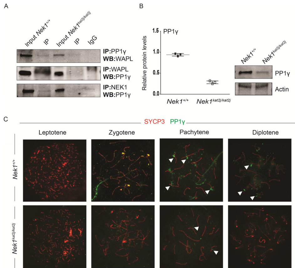
Figure 2. Loss of NEK1 induces a low protein levels and premature removal of PP1 \gamma from chromosome cores
