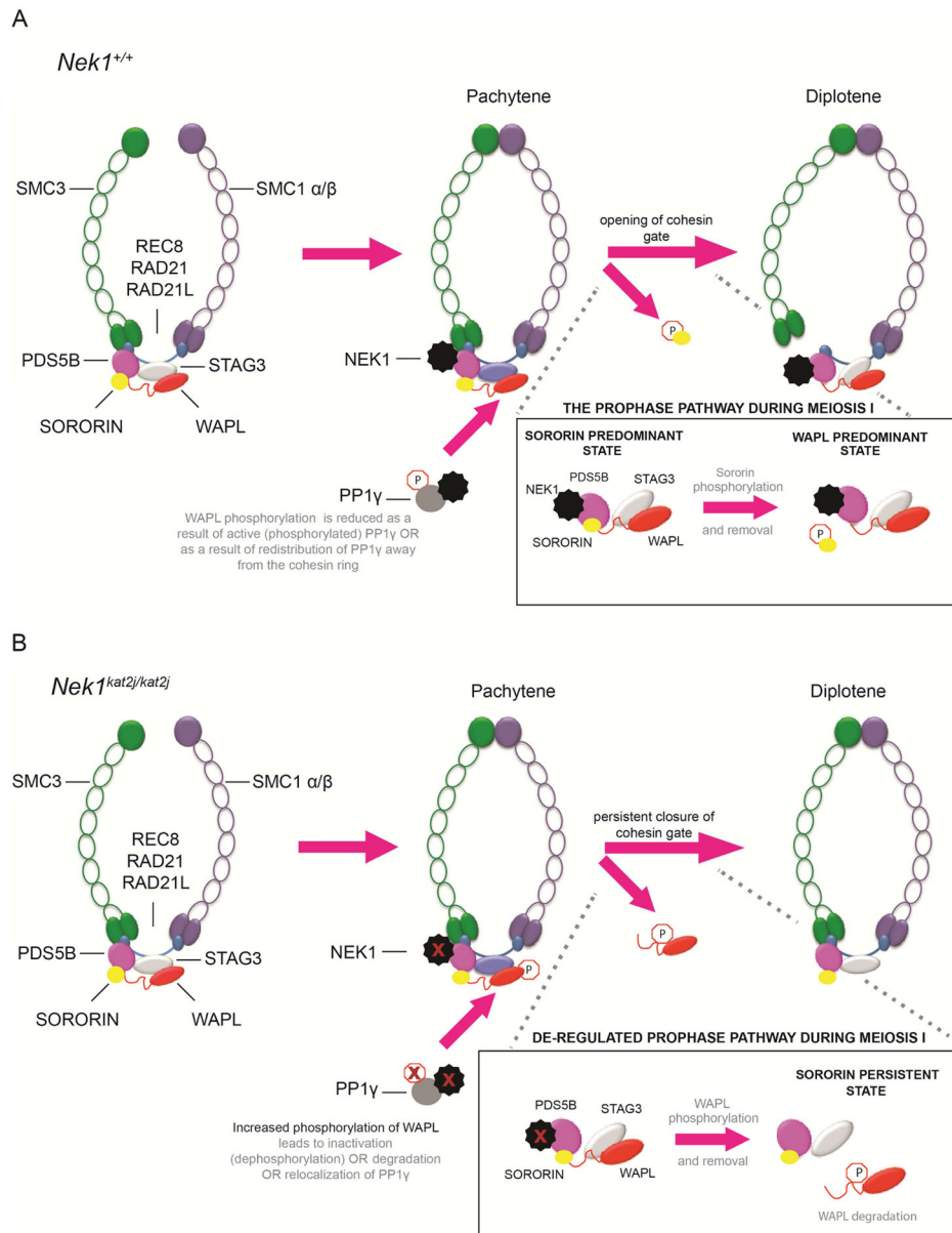
Figure 4. Model the role of NEK1 during meiotic prophase I
