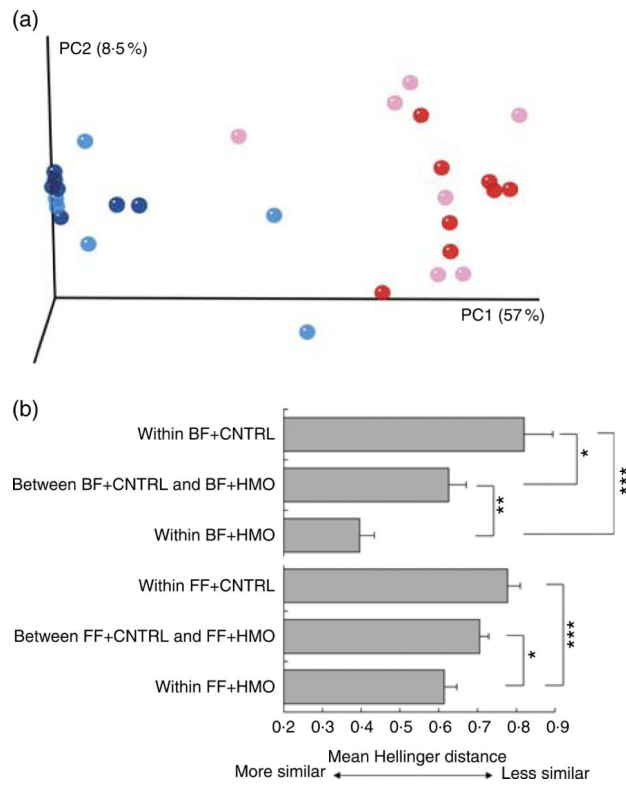
Fig. 3. \beta -Diversity analysis of the microbiota in mice treated with the human milk oligosaccharide (HMO) 2'-fucosyllactose. (a, b) \beta -Diversity analysis of the microbiota of the indicated treatment groups. Differences in \beta -diversity were evaluated using the Mann-Whitney U test. BF, breast-fed; CNTRL, control; FF, formula fed. * P < 0.05 ; ** P < 0.01 ; *** P < 0.001 . ●, BF + CNTRL; ●, BF + HMO; ●, FF + CNTRL; ●, FF + HMO. PC1, principal component 1; PC2, principal component 2.
