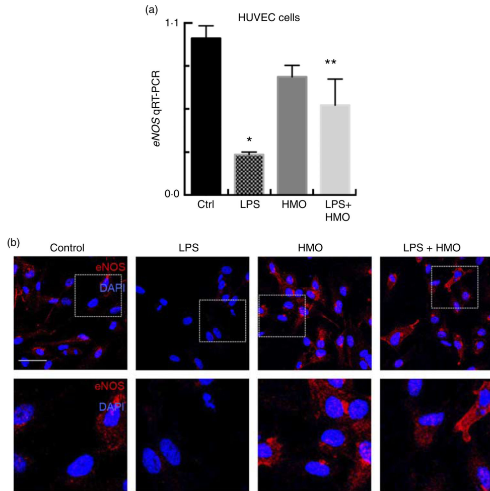
Fig. 7. Expression of endothelial nitric oxide synthase (eNOS) is enhanced by the human milk oligosaccharide (HMO) 2'-fucosyllactose in HUV-EC-C (HUVEC). (a) eNOS mRNA by quantitative real-time PCR (qRT-PCR) from HUVEC in the indicated treatment groups: vehicle control (Ctrl), lipopolysaccharide (LPS), HMO alone (HMO) and LPS with HMO (LPS + HMO) relative to the housekeeping gene RPL0 . (b) Representative confocal micrographs of HUVEC with the indicated treatment groups stained for eNOS (red) and 4,6-diamidino-2-phenylindole, dihydrochloride (DAPI) (blue). * P < 0.05 v. vehicle control, ** P < 0.05 v. LPS. Values are means with their standard errors. Scale bar is 10 \mu m. Results representative of three separate experiments with over 50 high power fields per group imaged.
