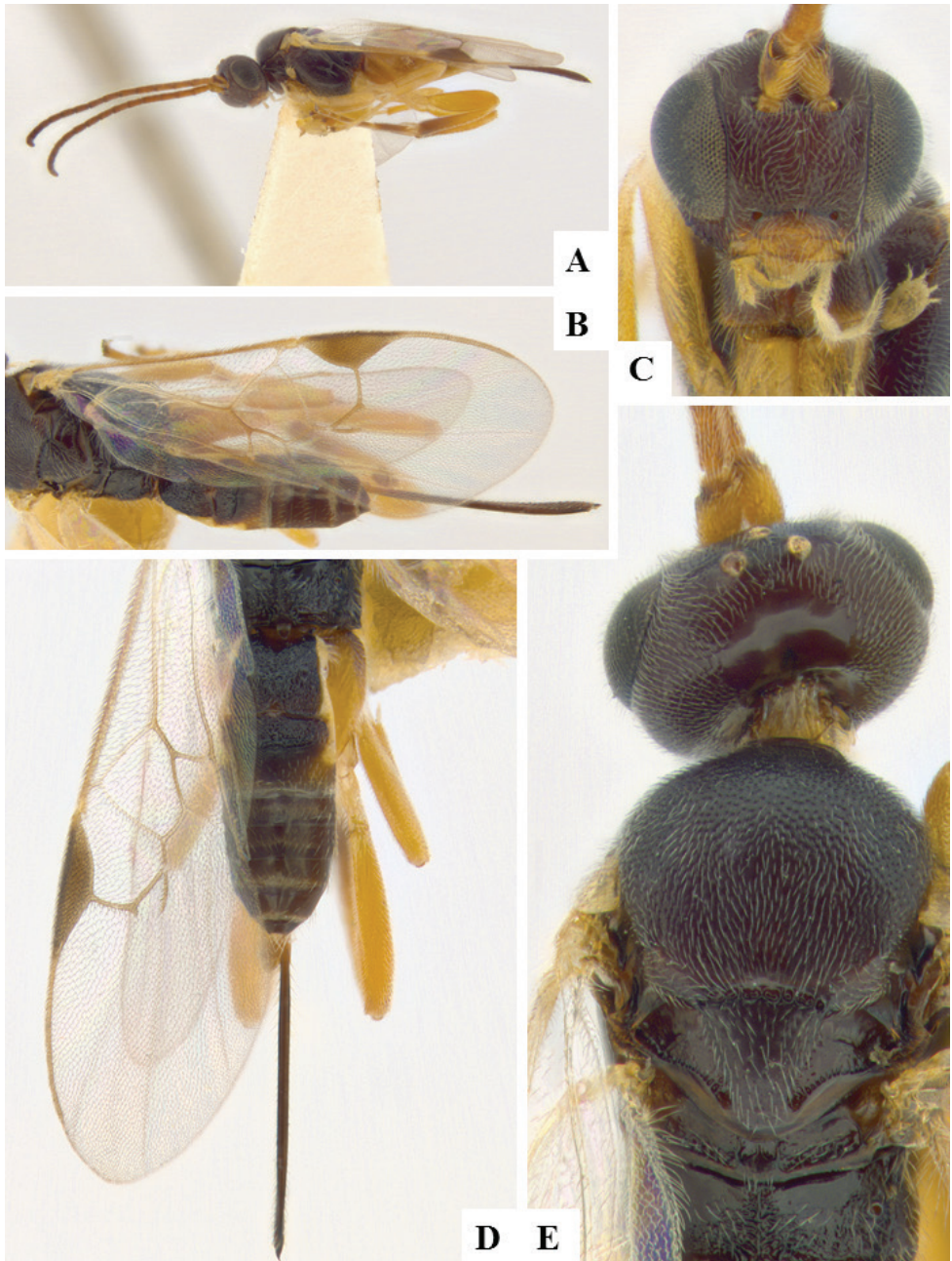
Figure 12. Choeras consimilis . A Habitus, lateral B Wings C Head, frontal D Metasoma dorsal E Head and mesosoma, dorsal.
