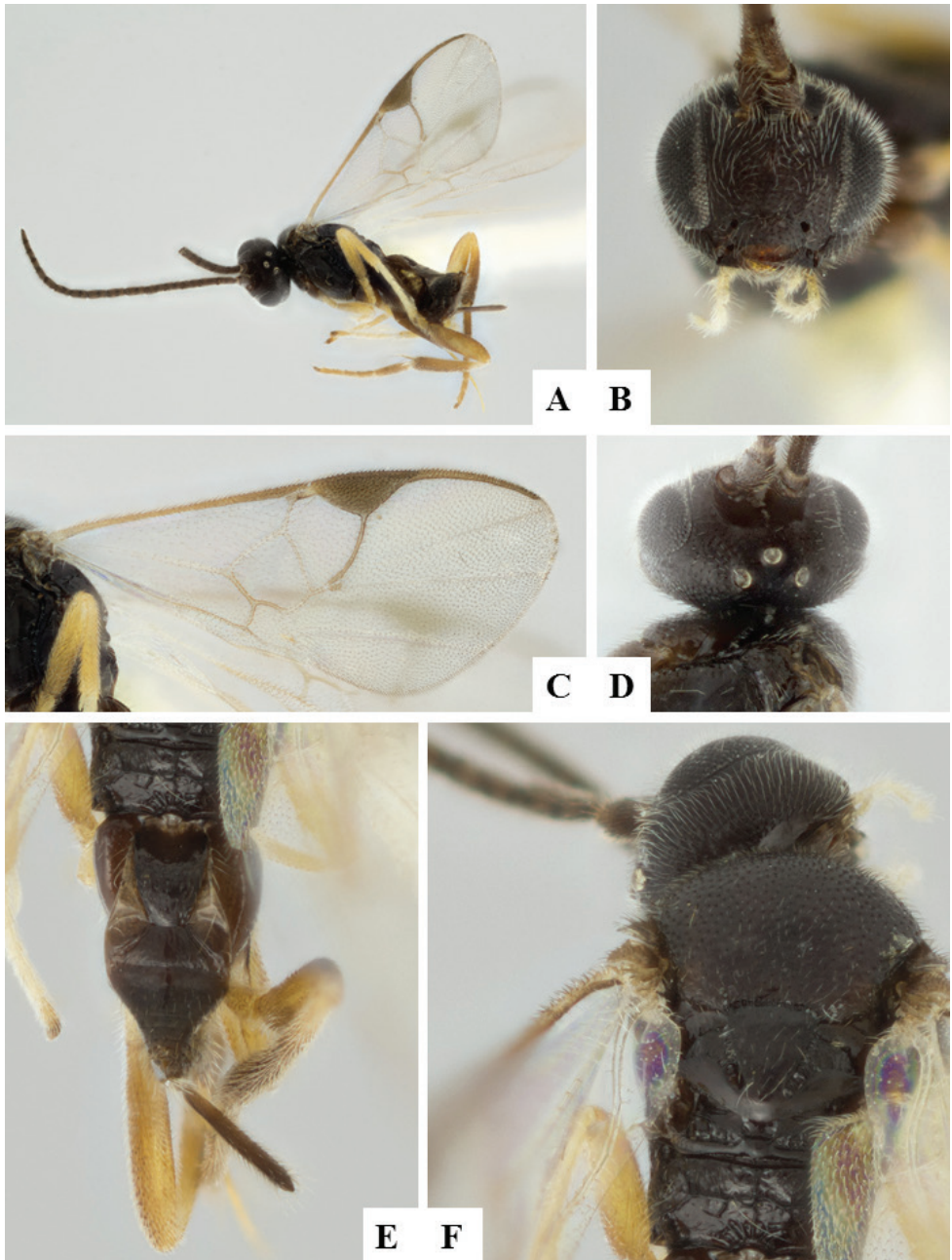
Figure 13. Clarkinella canadensis . A Habitus, lateral B Head, frontal C Wings D Head dorsal E Meta-soma, dorsal F Head and mesosoma, dorsal.
