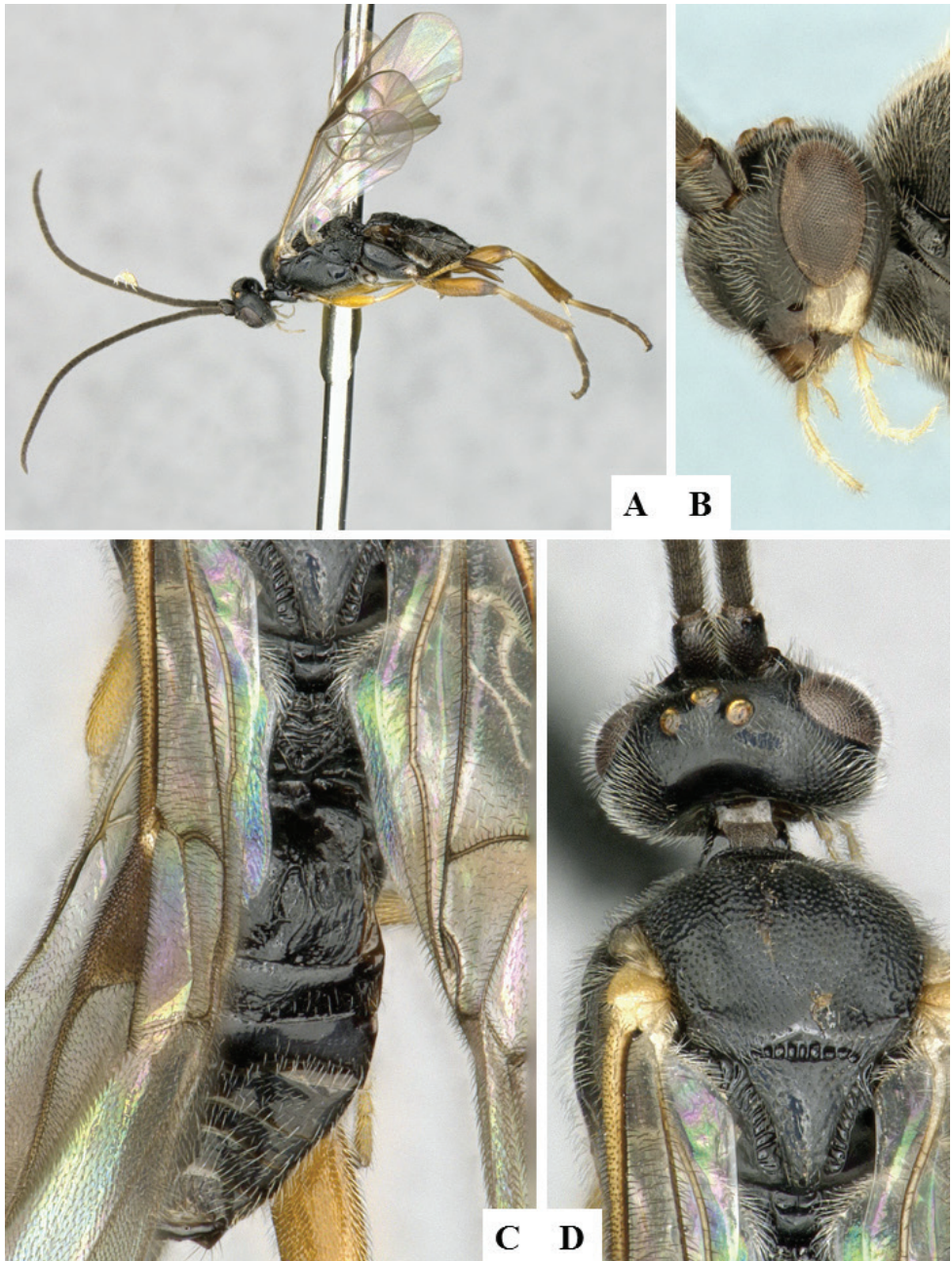
Figure 5. Alphonelton winniewertzae . A - Habitus, lateral B Head, lateral C Metasoma, dorsal D Head and mesosoma (partially), dorsal.
