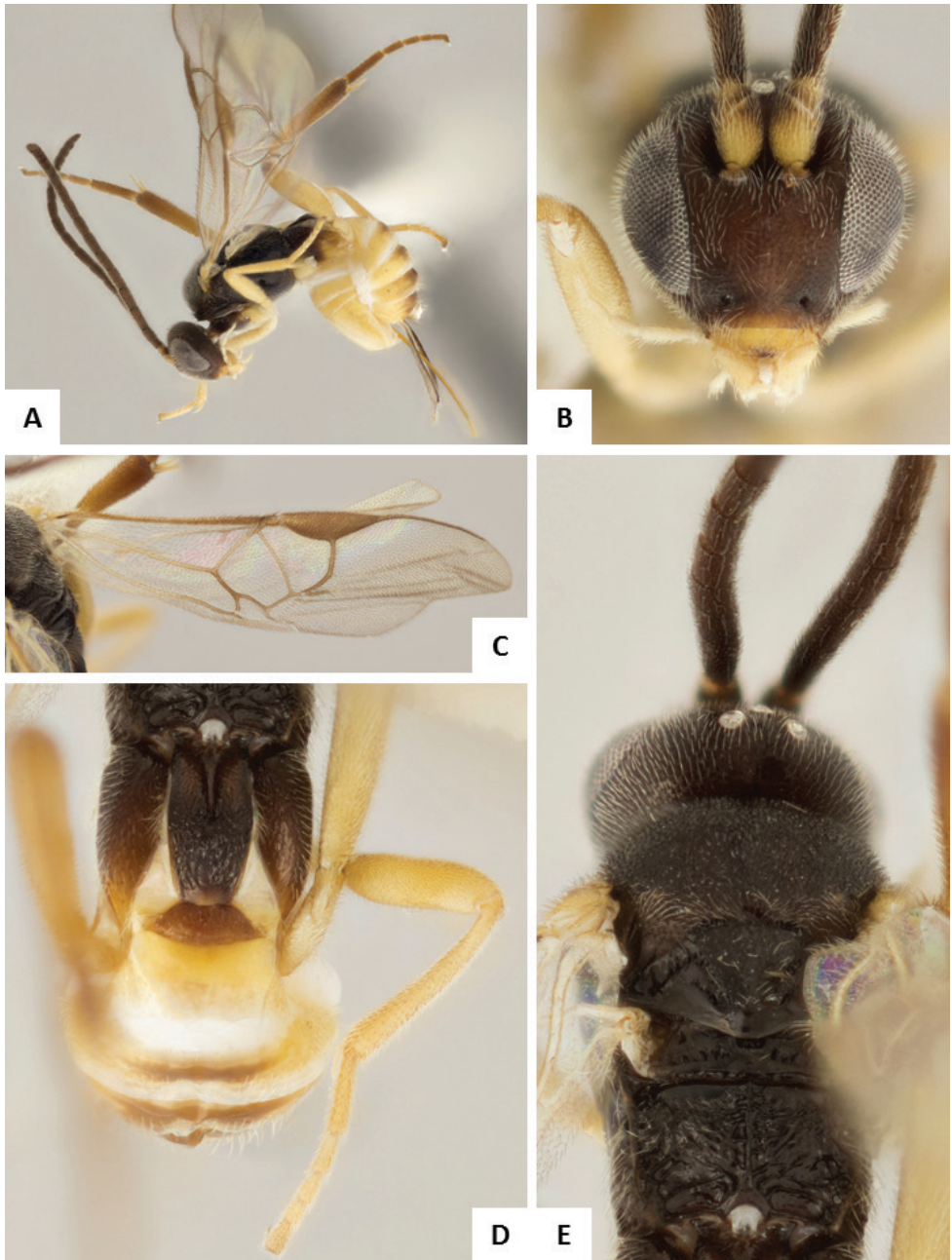
Figure 38. Pseudapanteles gouleti . A Habitus, lateral B Head, frontal C Wings D Metasoma, dorsal E Head and mesosoma, dorsal.
