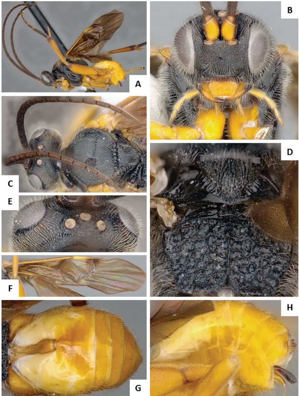
Figure 37. Protomicroplitis calliptera . A Habitus, lateral B Head, frontal C Head and mesosoma (partially), dorsal D Propodeum E Head, dorsal F Wings G Metasoma, dorsal H Metasoma, lateral.
