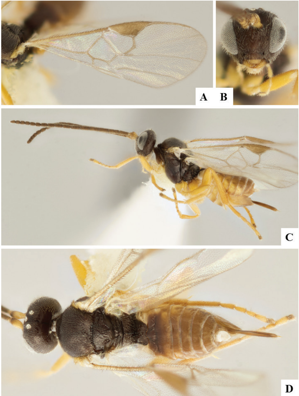
Figure 27. Lathrapanteles heleios . A Wings B Head, frontal C Habitus, lateral D Habitus, dorsal.
