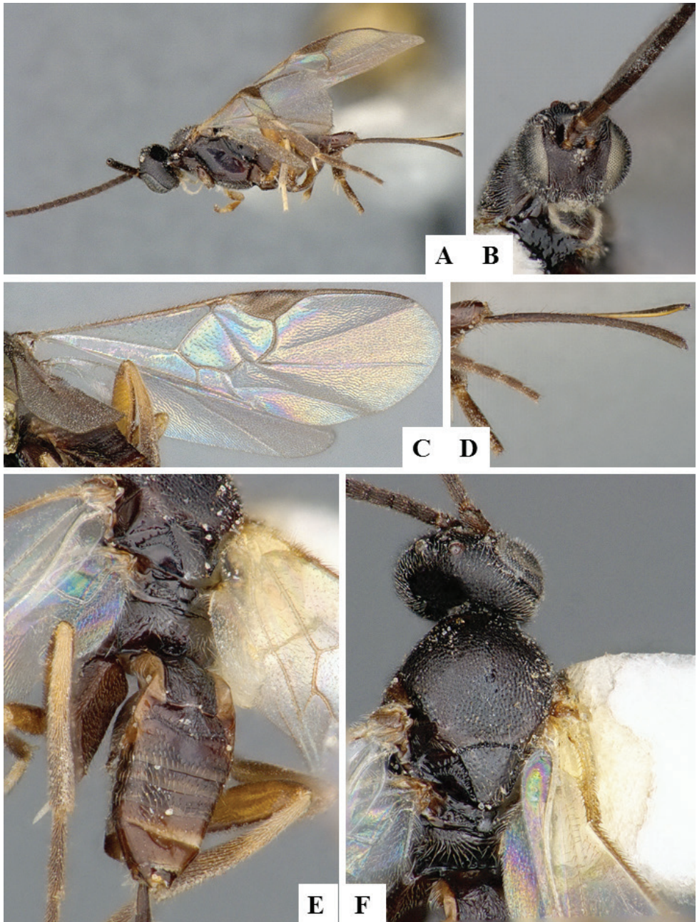
Figure 22. Dolichogenidea renaulti . A Habitus, lateral B Head, frontal C Wings D Ovipositor sheaths E Mesosoma (partially) and metasoma, dorsal F Head and mesosoma, dorsal.
