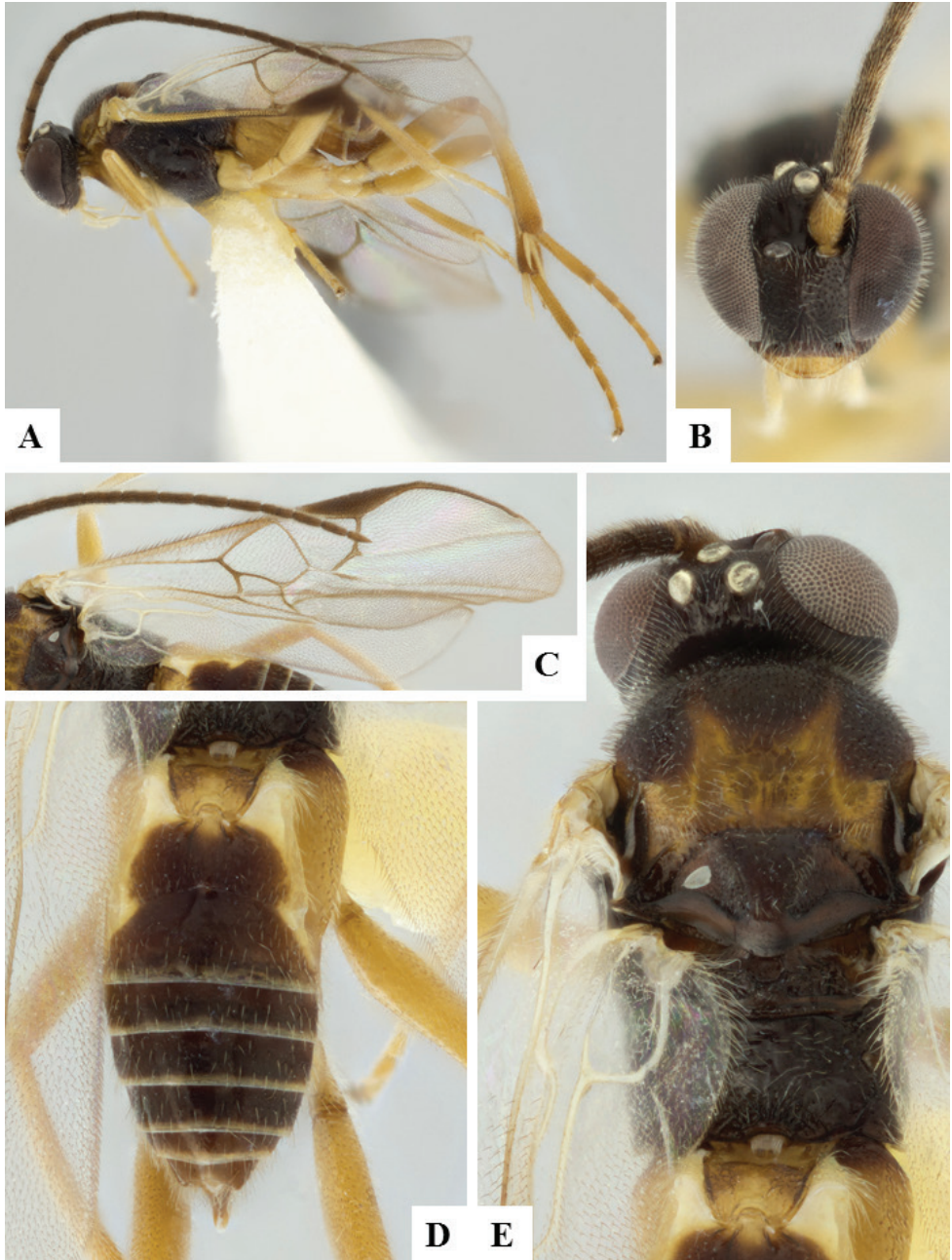
Figure 18. Distatrix carolinae . A Habitus, lateral B Head, frontal C Wings D Metasoma, dorsal E Head and mesosoma, dorsal.
