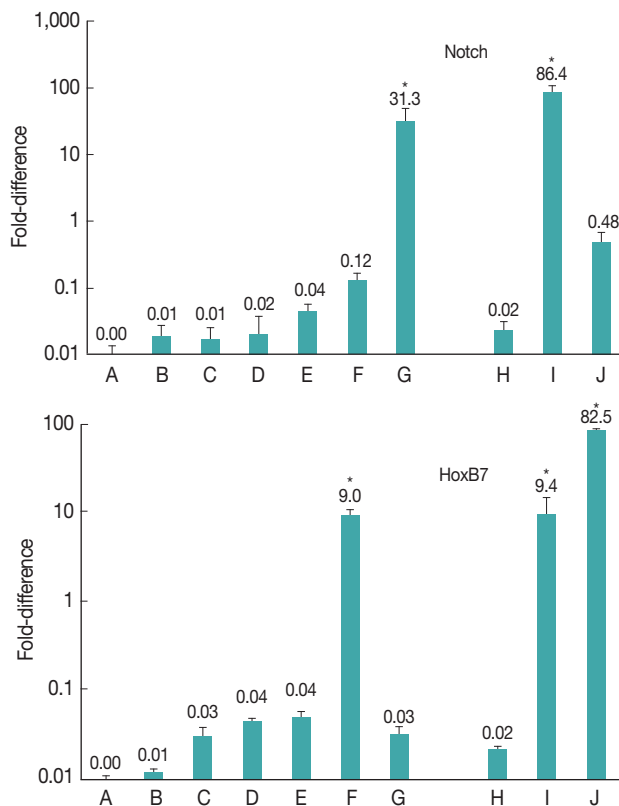
Fig. 2. Expression of Notch and HoxB7 genes in developmental stages of E. granulosus in vitro and in vivo. (A) Evaginated protoscoleces. (B) Excretory-canal-and-bladder-formation. (C) First-proglottid-formation. (D) Second proglottid-formation. (E) Testes-and-genital-pore-appearance. (F) Third-or-more-proglottid. (G) Microcysts in monophasic media. (H) Intact protoscoleces. (I) Germinal layer of hydatid cyst. (J) Adult worms isolated from a dog. *statistically significant ( P < 0.05 ).
