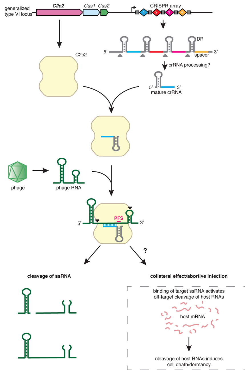
Figure 7. C2c2 as a putative RNA-targeting prokaryotic immune system The C2c2-crRNA complex recognizes target RNA via base pairing with the cognate protospacer and cleaves the target RNA. In addition, binding of the target RNA by C2c2-crRNA activates a non-specific RNase activity which may lead to promiscuous cleavage of RNAs without complementarity to the crRNA guide sequence. Through this non-specific RNase activity, C2c2 may also cause abortive infection via programmed cell death or dormancy induction.
