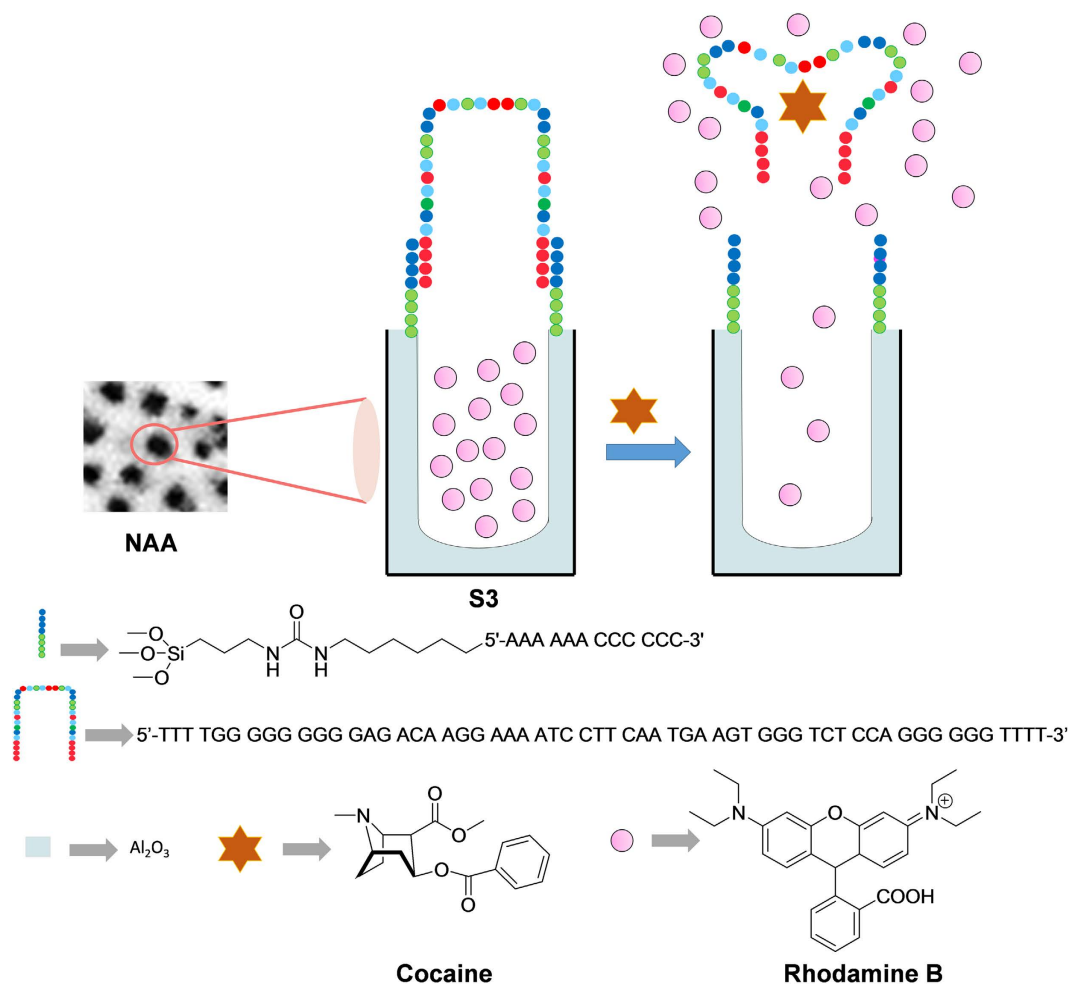
Figure 1. Scheme of the gated NAA support S3 capped with the selected aptamer. Delivery of the entrapped dye (rhodamine B) is selectively accomplished in the presence of cocaine.
