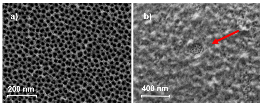
Figure 2. FESEM images of (a) parent NAA support and (b) support S3. Arrow indicates a certain area where the porous framework can be seen below the organic layer.
