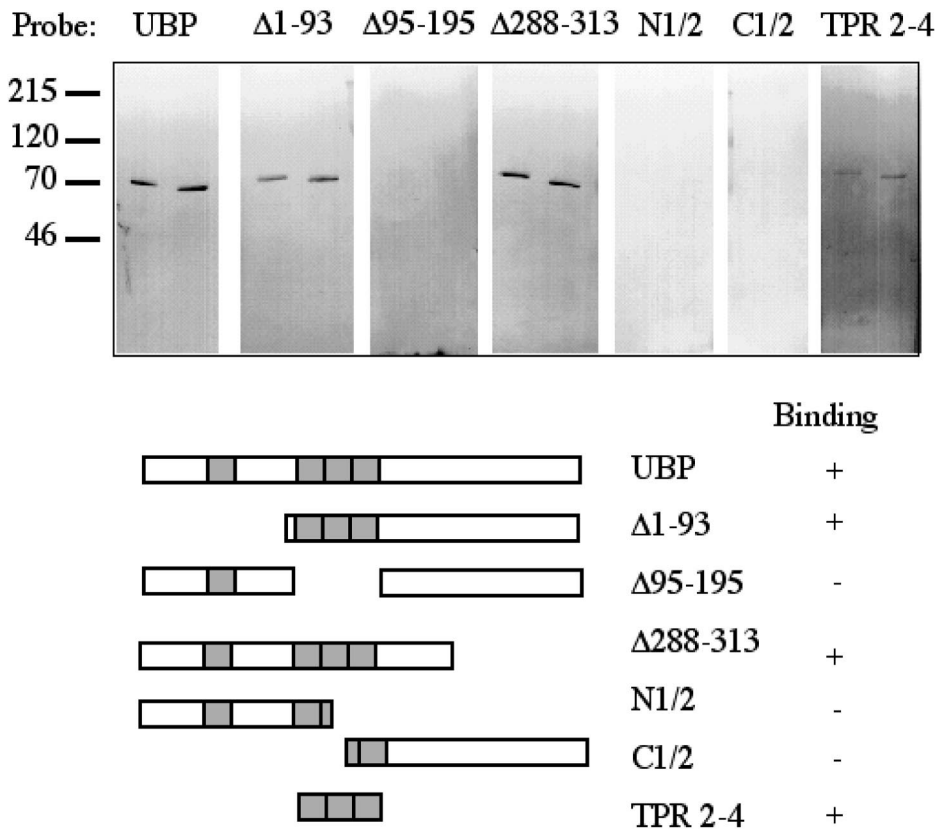
Fig 2. Mapping of the small glutamine-rich protein (SGT)/viral protein U-binding protein (UBP)/Hs70 interaction, where Hs70 represents heat shock protein (Hsp) 70 and its constitutive counterpart, Hsc70. Seven identical sets of blots containing Hsc70 and Hsp70 were subjected to SGT/UBP Far-Western analysis. The blots were probed with GST fusions as indicated: full-length SGT/UBP, \Delta 1–93, \Delta 95–195, \Delta 288–313, N1/2 (amino acids [a.a.] 1–145), C1/2 (a.a. 145–313), and tetratricopeptide repeats 2–4 (a.a. 95–195). The numbers to the left of the blots indicate the molecular weights in kilodaltons. The diagram below the blots indicates regions of SGT/UBP contained in each fusion construct. The column to the right summarizes the results; a plus symbol indicates binding and a minus symbol indicates no binding.
