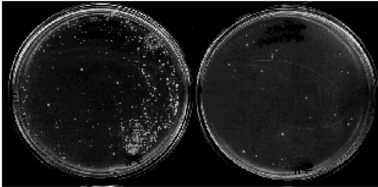
Fig 6. Deletion mutants of small glutamine-rich protein/viral protein U-binding protein (SGT/UBP) in Saccharomyces cerevisiae are defective for recovery from severe heat shock. Wild type (wt) or SGT/UBP deletion strains were subject to heat shock at 55°C for 1 hour and then plated at appropriate dilutions to rich media. The plates at the top of the bar graph show representative surviving colonies from wild type or SGT/UBP-deletion strains. The number of surviving colonies was counted, and the data were expressed as the percent total survivor, with wild type SGT/UBP set to 100%.
