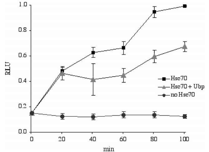
Fig 4. Small glutamine-rich protein/viral protein U-binding protein (SGT/UBP) inhibits refolding of denatured firefly luciferase dependent on the constitutive counterpart, Hsc70, of heat shock protein (Hsp) 70. Heat-denatured luciferase was incubated with Hsc70 (square), Hsc70 and SGT/UBP, or no Hsc70 (circle). Luciferase activity was quantified using a luminometer. Data are plotted as the relative light units as a function of time from 0 minutes to 100 minutes.
