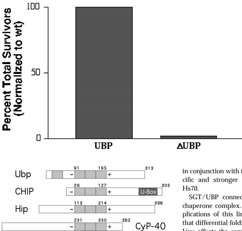
Fig 7. Comparison of several tetratricopeptide repeat-containing co-chaperones.
