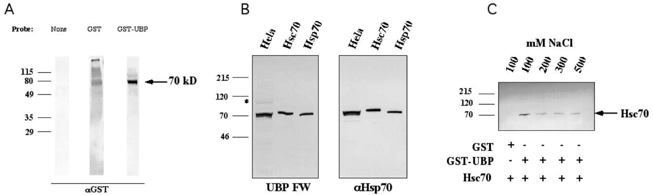
Fig 1. Small glutamine-rich protein/viral protein U-binding protein (SGT/UBP) binds directly to heat shock protein 70 (Hsp70) and its constitutive counterpart, Hsc70, with high affinity. (A) HeLa cell lysate (30 \mu g) was separated by sodium dodecyl sulfate–polyacrylamide gel electrophoresis in 3 identical lanes blotted to nitrocellulose and probed with no probe (none), GST alone, or GST-SGT/UBP. The Far-Western blot was then developed with anti-GST antibody to reveal bands that interact with SGT/UBP. The arrow to the right indicates a 70-kDa band detected by the GST-SGT/UBP fusion. The numbers to the left of each blot represent molecular weights in kilodaltons. (B) Identical blots containing 30 \mu g of HeLa lysate, 50 ng pure Hsc70, and 50 ng pure Hsp70, as indicated, were subjected to SGT/UBP Far-Western (SGT/UBP FW) or anti-Hsp70 Western analysis ( \alpha HSP70). The asterisk indicates the position of Hsp90, also detected in HeLa lysate by SGT/UBP Far-Western interaction. (C) Samples from the GST-SGT/UBP pull-down assay were analyzed by Western blot for the presence of Hsc70. At the bottom of the gel, the contents of each reaction are indicated by the plus symbols. The NaCl concentration of the washing buffer (100, 200, 300, and 500 mM) is indicated at the top of each lane. The arrow to the right of the blot indicates the position of the Hsc70 band.
