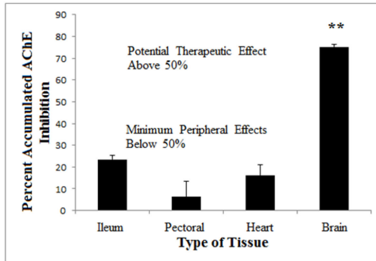
FIGURE TWO. Actual Accumulated AChE Inhibition in Rat Tissues after Three Weeks of Repeated Doses of MSF
