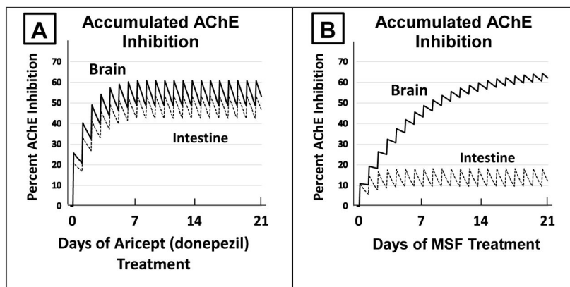
FIGURE ONE. Side-by-Side Computational Comparison of Expected Competitive versus Irreversible AChE Inhibition Through 21 Days of Treatment
