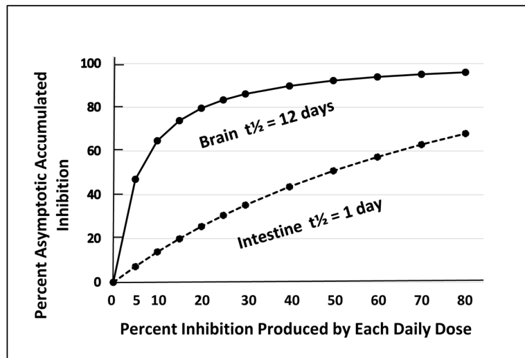
FIGURE FOUR. Hypothetical Relationship Between Dose Size and Accumulated Asymptotic Brain AChE Inhibition
