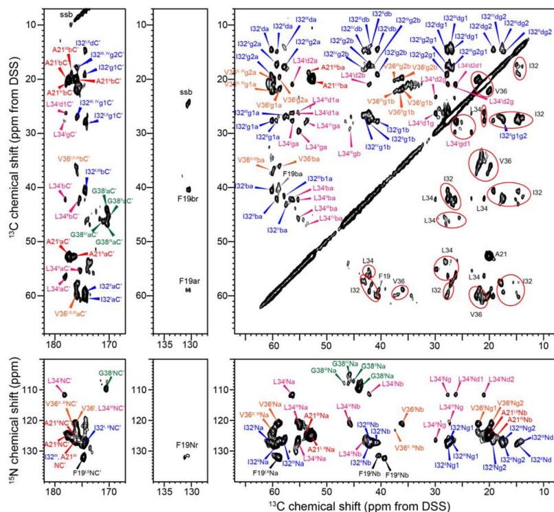
Figure 3. 2D correlation spectra of Arctic A \beta 40 (E22G) fibrils. (a) 2D ^{13}\text{C} - ^{13}\text{C} DARR spectrum with 50 ms mixing. For simplicity, assignments are given with lower-case letters for various carbons, and F19 aromatic carbons are designated by “r”. ssb denotes spinning sidebands. (b) 2D N(CA)CX ^{15}\text{N} - ^{13}\text{C} correlation spectrum. Two to four sets of chemical shifts (denoted by subscripts I – IV) are identified for all labeled residues, indicating extensive structural polymorphism. Ellipses guide the eye for chemical shift multiplicity. The DARR spectrum was processed using a QSINE window function with \text{SSB} = 2.5 , and were plotted with Topspin parameters \text{lev}0 = 4 , \text{toptev} = 90 and \text{nlev} = 16 . 2D N(CA)CX spectrum was processed using a Gaussian window function with \text{LB} = -10 Hz and \text{GB} = 0.05 , and was plotted using \text{lev}0 = 5 , \text{toptev} = 80 and \text{nlev} = 16 .
