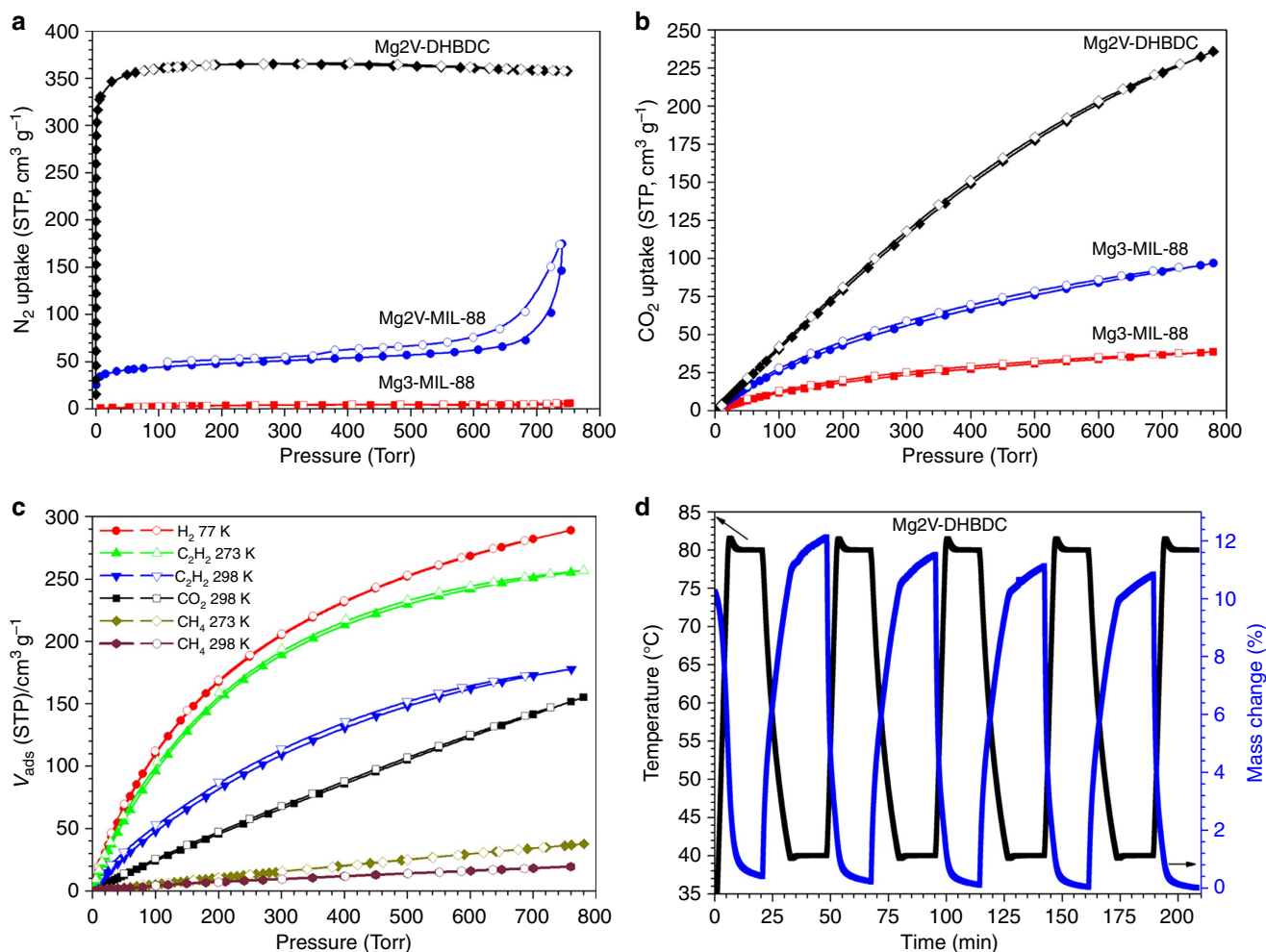
Figure 2 | Gas sorption study on MIL-88 and pacs-MOF compounds. (a) N 2 sorption isotherm at 77 K. (b) CO 2 sorption at 273 K. (c) H 2 (77 K), CO 2 (298 K), CH 4 (273 and 298 K), and C 2 H 2 (273 and 298 K) adsorption isotherms. (d) Repeated adsorption-desorption kinetics between a 15: 85 CO 2 /N 2 (v/v) flow at 313 K and a pure N 2 flow at 353 K.
