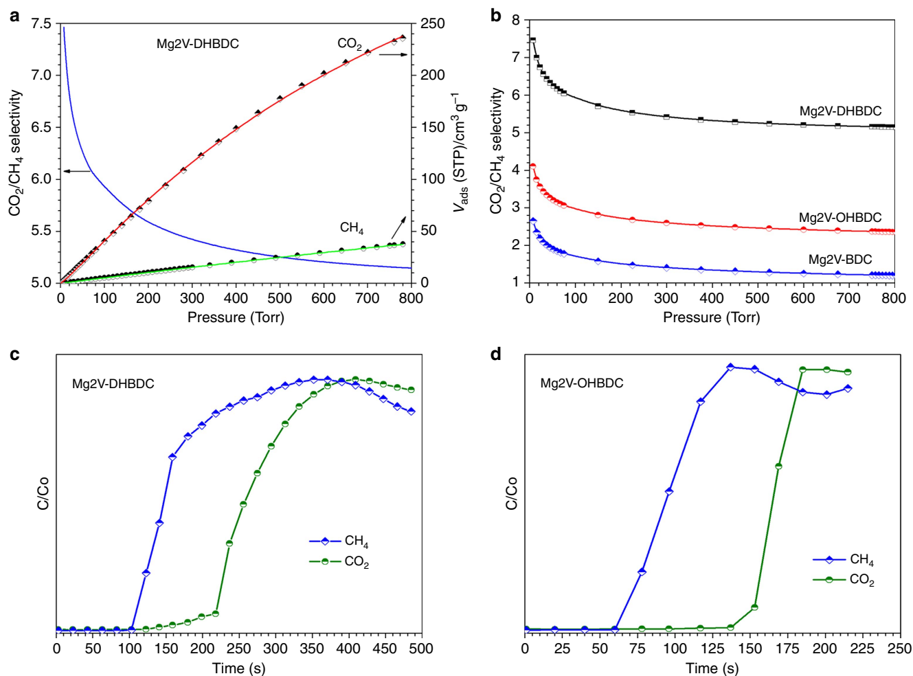
Figure 3 | The CO 2 /CH 4 selectivity evaluation for Mg 2 V-MOFs. (a,b) Adsorption selectivity predicted by IAST for CO 2 (50%) over CH 4 (50%) at 273 K. (c,d) Breakthrough curves for the separation of a 0.15:0.85 (v/v) 16 ml min -1 flow of CO 2 /CH 4 mixture at 296 K.
