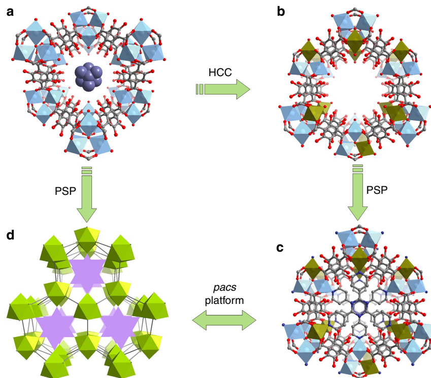
Figure 1 | Stepwise design of the pacs -MOF platform. (a) Anionic framework of Mg 3 -MIL-88 with the charge-balancing [(CH 3 ) 2 NH 2 ] + cations simplified as blue balls. (b) V 3+ -containing neutral framework of Mg 2 V-MIL-88 . (c) Pore space partitioning through TPT insertion in Mg 2 V-DHBDC . (d) Polyhedral drawing of PSP through TPT insertion in Mg 3 -DHBDC . TPT = 2,4,6-tri(4-pyridinyl)-1,3,5-triazine.
