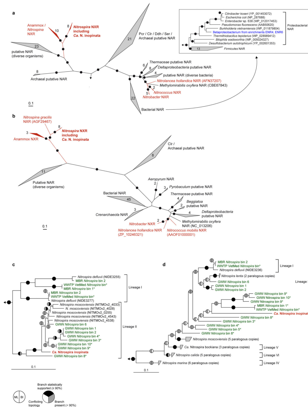
Extended Data Figure 5. Phylogeny of NXR from Ca. N. inopinata and related proteins. a,b , Maximum likelihood trees showing the alpha ( a ) and beta ( b ) subunits of selected enzymes from the DMSO reductase type II family. Names of validated enzymes are indicated (Clr, chlorate reductase; Ddh, dimethylsulfide dehydrogenase; NAR, nitrate reductase; NXR, nitrite oxidoreductase; Pcr, perchlorate reductase; Ser, selenate reductase). More distantly related molybdoenzymes were used as outgroup. Black dots on branches indicate high maximum likelihood bootstrap support ( \geq 90\% ; 1,000 iterations). Known NXR forms are highlighted in red. The inset in ( a ) contains a subtree, which shows the
