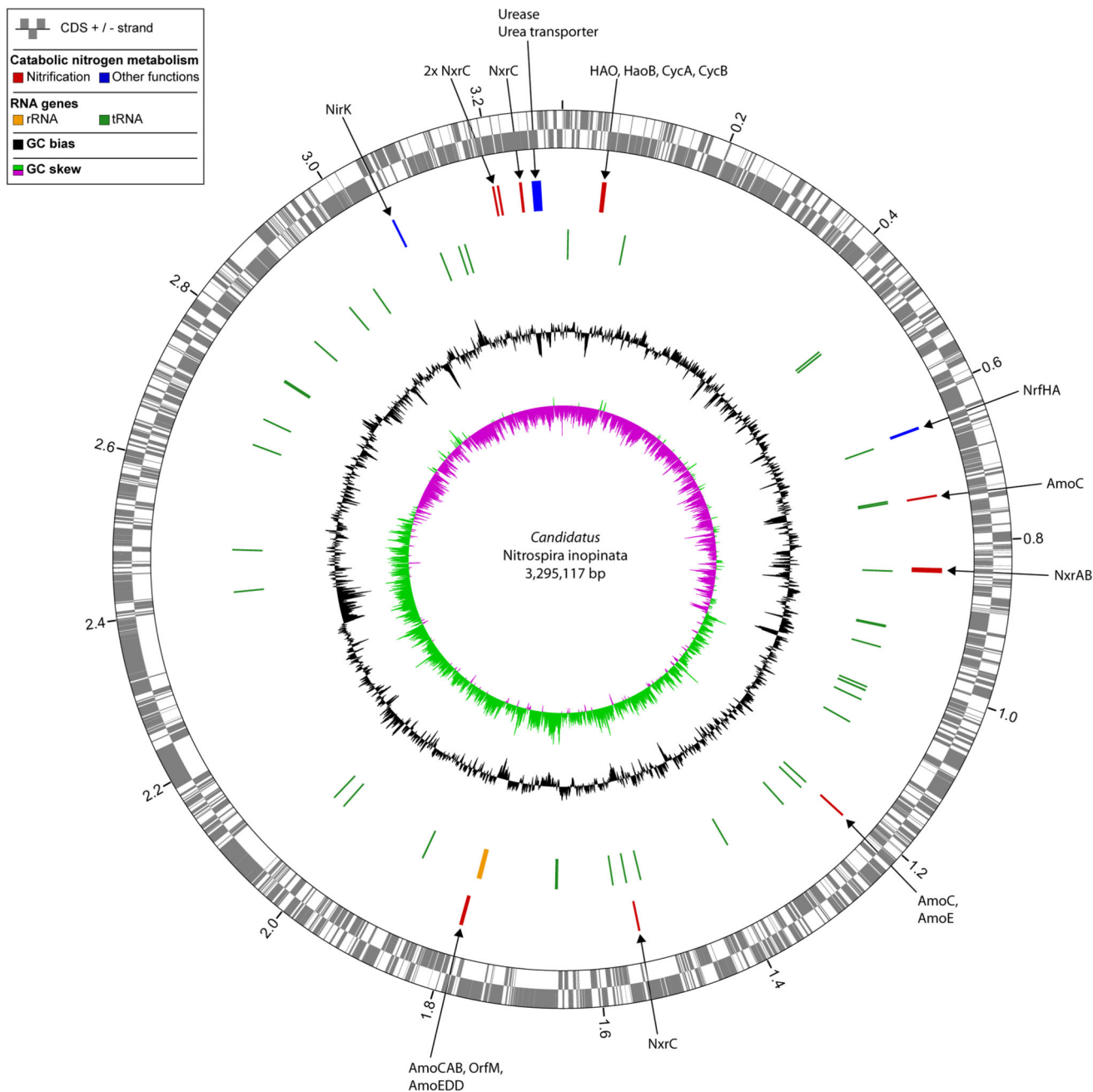
Extended Data Figure 3. Circular representation of the Ca. N. inopinata chromosome. Predicted coding sequences (CDS; rings 1+2), genes of enzymes involved in nitrification and other pathways of catabolic nitrogen metabolism (ring 3), RNA genes (ring 4), and local nucleotide composition measures (rings 5+6) are shown. Very short features were enlarged to enhance visibility. Clustered genes, such as several tRNA genes, may appear as one line due to space limitations. The tick interval is 0.2 Mbp. Abbreviations: Amo, ammonia monooxygenase; HAO, hydroxylamine dehydrogenase; CycA and CycB, tetraheme c -type cytochromes that form the hydroxylamine ubiquinone redox module together with HAO;
