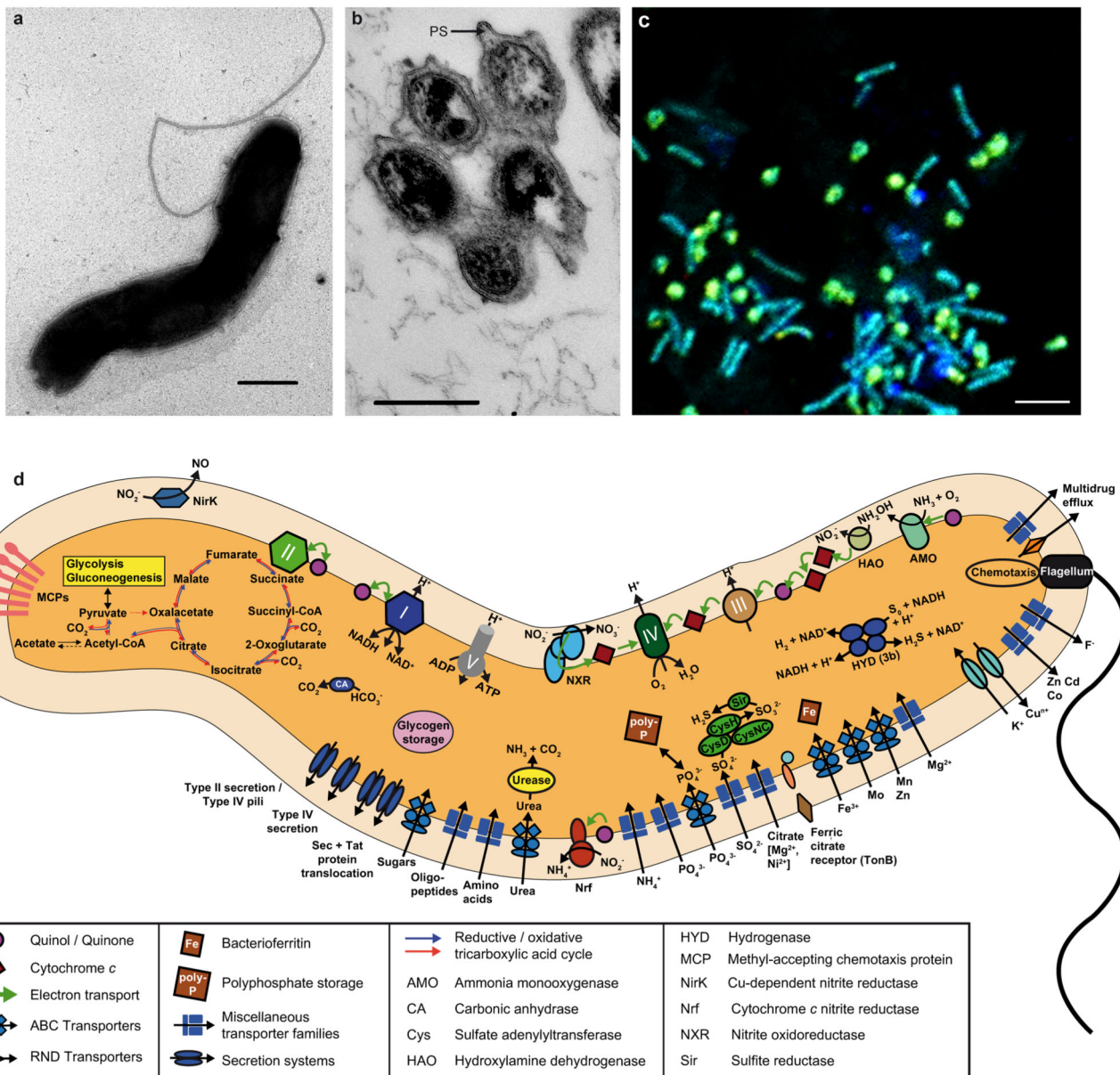
Extended Data Figure 1. Photomicrographs and cell diagram of Ca. Nitrospira inopinata .
