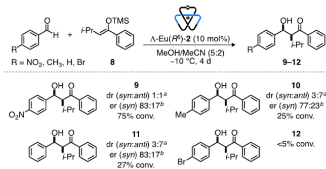
Figure 4. Chiral trefoil knot Λ-Eu(R 6 )-2(CF 3 SO 3 ) 3 -catalyzed asymmetric Mukaiyama aldol reactions. Reaction conditions: 1.0 equiv of aldehyde and 1.5 equiv of trimethyl(3-methyl-1-phenylbutenyloxy)silane at -10\text{ }^{\circ}\text{C} for 4 days. a Determined by ^1\text{H} NMR analysis. b Determined by chiral HPLC. In all cases the relative stereochemistry of the most enantioenriched diastereomer is shown.
