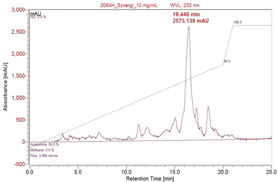
Figure 2. HPLC chromatogram of 2064H Reverse Phase HPLC (100 \mu L injection; 10 mg/mL); Major peak at 16.440 min and 2573 mAU was isolated as pure compound 2064H3.
