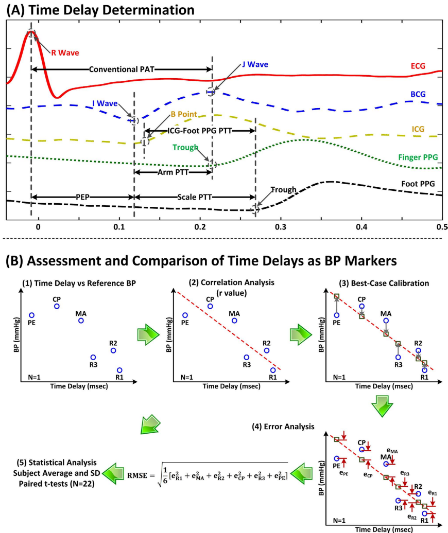
Figure 2. Data analysis for comparing scale PTT to conventional PAT as markers of BP in humans.
