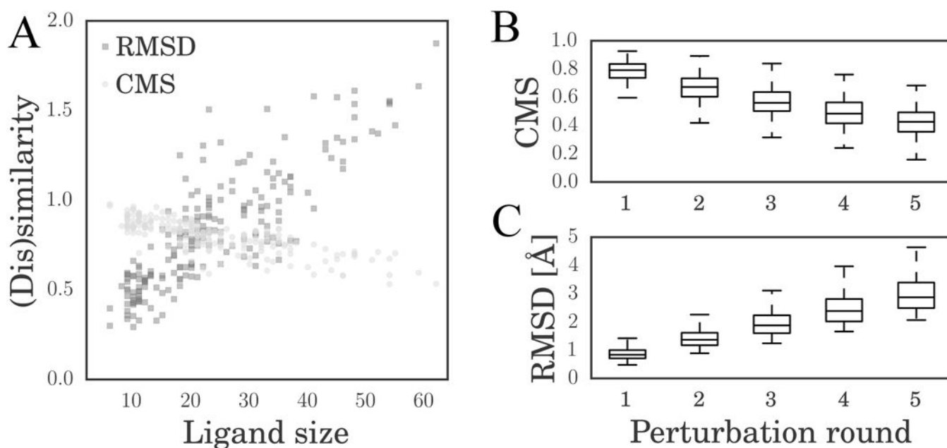
Figure 4. Comparison of RMSD and CMS in the perturbation experiment
