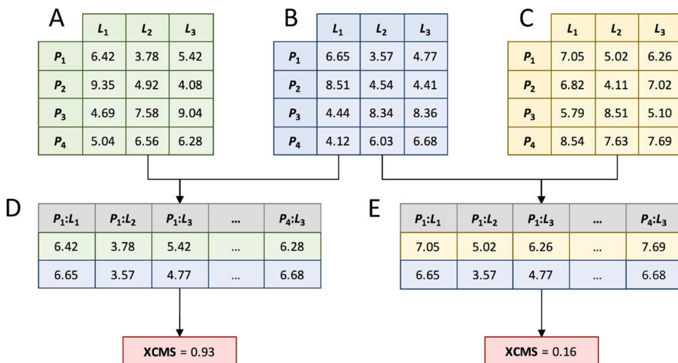
Figure 2. Calculation of the eXtended Contact Mode Score (XCMS)
