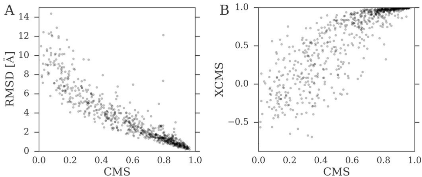
Figure 8. Correlation between RMSD, CMS, and XCMS
