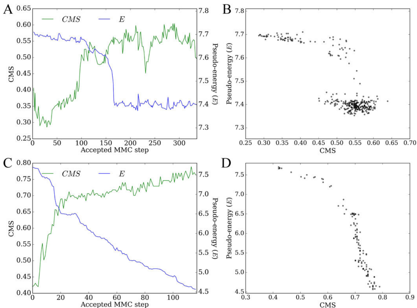
Figure 5. Analysis of docking trajectories with the CMS
