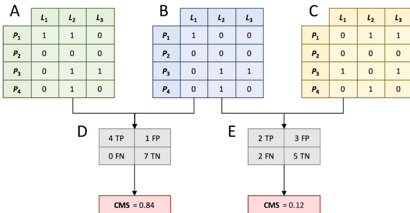
Figure 1. Calculation of the Contact Mode Score (CMS)
