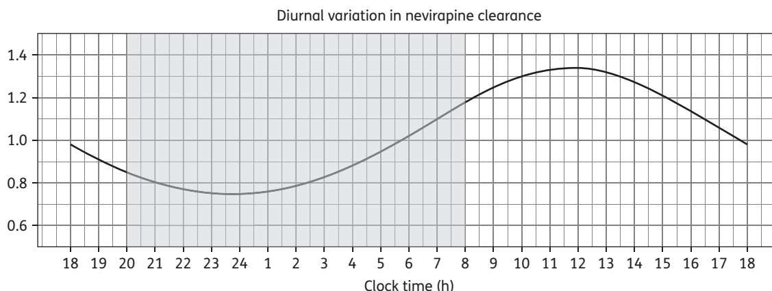
Figure 2. Diurnal variation in nevirapine intrinsic clearance detected by the model, presented over 24 h. The shaded area corresponds to night-time (20.00–08.00 h).
