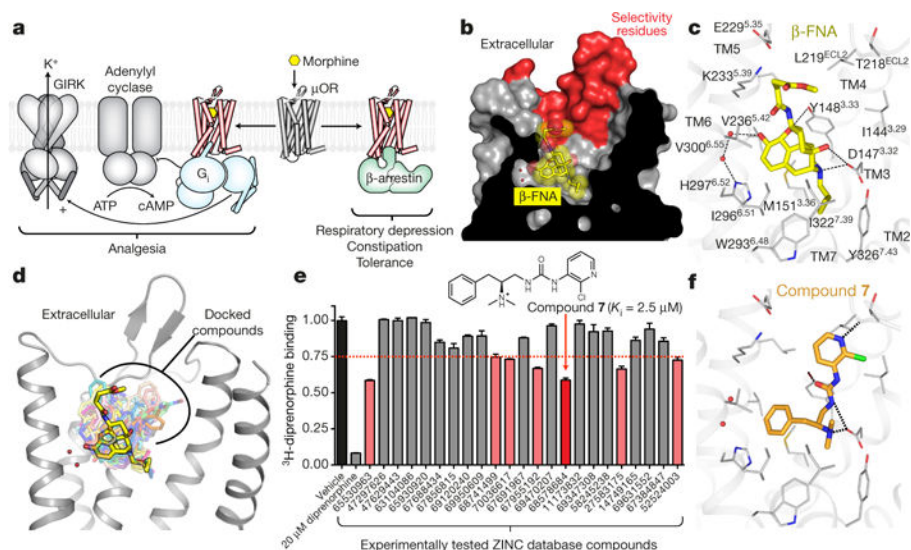
Figure 1. Structure based ligand discovery for the \mu OR
