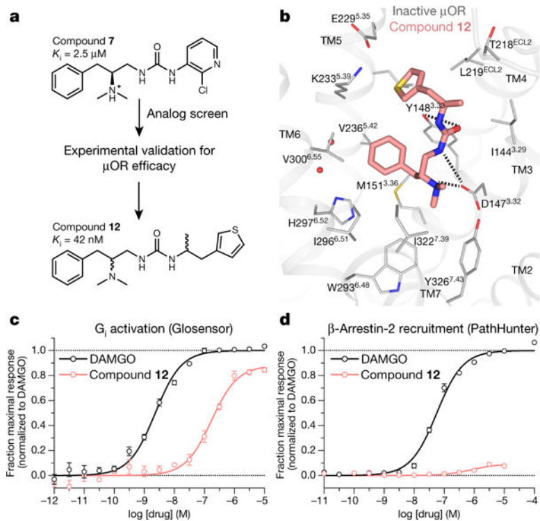
Figure 2. Discovery of a novel G_{i/o} -biased \mu OR agonist
