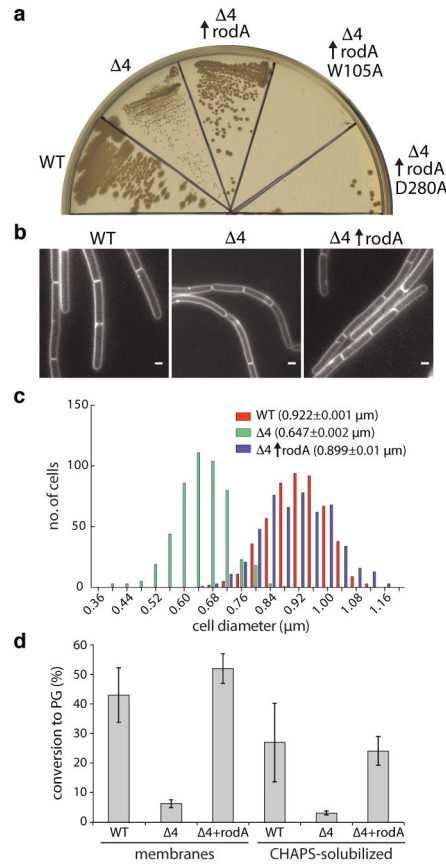
Fig. 3. RodA overexpression partially suppresses the phenotypes of the \Delta 4 mutant a , Suppression of growth defects and b , morphological defects in the \Delta 4 mutant by rodA overexpression, representative of 3 biological replicates. Scale bar indicates 1 \mu\text{m} . c , Histogram of cell diameters for the indicated strains, n=500 . Average diameter is indicated in parenthesis. d , PGT activity catalyzed by membranes and CHAPS-solubilized membrane proteins derived from the indicated strains. Data show the mean of 3 biological replicates, error bars denote standard error of the mean (s.e.m.).
