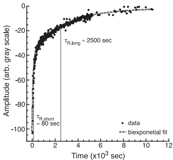
Fig. 2. Representative biexponential fluorescence recovery curve for acrylodan-labeled four-repeat tau (circles). Recovery curves for all types of samples overlap this data. The fit (dashed line) yields a short time constant, \approx 80 sec, corresponding to diffusion of unbound tau around the MTs or fast dissociation of loosely bound tau. The long time constant, \approx 2,500 sec, corresponds to the characteristic dissociation time for tau.
