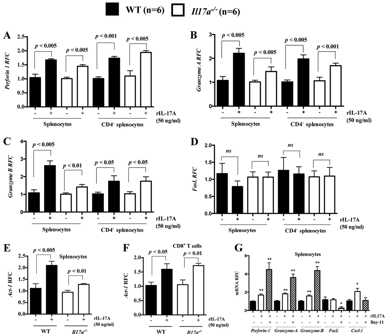
FIG 6 IL-17A promotes expression of cytotoxic-mediator genes independently of CD4 + T cells. (A to D) Seven- to 9-week-old WT (C57BL/6J) and Il17a -/- mice ( n = 6 mice/group) were infected (i.p.) with 100 PFU of WNV and sacrificed at 8 dpi to isolate splenocytes and CD8 + T cells. Splenocytes or CD4 + T cell-depleted splenocytes (CD4 - splenocytes) were cultured with or without recombinant mouse IL-17A (rIL17A) (50 ng/ml) for 24 h ex vivo , and RFC of transcripts of perforin-1 (A), granzyme A (B), granzyme B (C), and FasL (D) was measured by qPCR (normalized to cellular \beta -actin mRNA). (E and F) Splenocytes (E) or purified CD8 + T cells (F) were cultured ex vivo with or without recombinant IL-17A (50 ng/ml) for 24 h, and expression (RFC) of Act-1 was by measured qPCR. (G) RFC of indicated genes in splenocytes cultured ex vivo for 24 h with or without rIL17A (50 ng/ml) in the presence of Bay-11-7082 (4 \mu M) or dimethyl sulfoxide (DMSO) as a vehicle control (<0.05%). All the data (means and SEM) represent the results of two independent experiments ( n = 3 mice/group) compared by two-tailed Student t tests. (A to F) All the data from WT and Il17a -/- mice were normalized to the respective mock-treated controls. *, P < 0.05; **, P < 0.005; ns , not significant ( P > 0.05).
