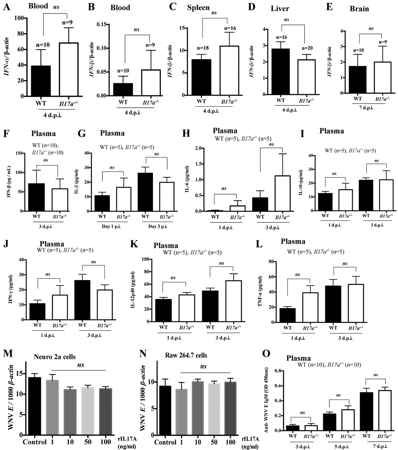
FIG 4 Antiviral, inflammatory, and antibody responses of Il17a -/- mice during WNV infection. Seven- to 9-week-old WT (C57BL/6J) and Il17a -/- mice were infected (i.p.) with 1,000 PFU of WNV. Blood, plasma, and tissue samples were collected at the indicated time points for cytokine and anti-WNV-E IgM measurement. (A to E) Expression of Ifn- \alpha gene transcripts in blood (A) and expression of Ifn- \beta gene transcripts in blood (B), spleen (C), liver (D), and brain (E) were measured by qPCR (normalized to cellular \beta -actin mRNA). (F to L) Protein levels of IFN- \beta , IL-1 \beta , IL-6, IL-10, IFN- \gamma , IL-12p40, and TNF- \alpha in plasma were measured by ELISA. (M and N) Replication of WNV was analyzed by qPCR in Raw 264.7 (M) and Neuro 2a (N) cells that were pretreated with mouse recombinant IL-17A (1 to 100 ng/ml) for 6 h, followed by infection with WNV (MOI = 1) for 24 h. (O) Anti-WNV-E IgM in plasma was measured by ELISA. The data (means and SEM) represent the results of at least two independent experiments performed in triplicate and analyzed by one-way ANOVA (M and N) or two-tailed Student t tests (A to L and O); ns , no significant difference ( P > 0.05).
