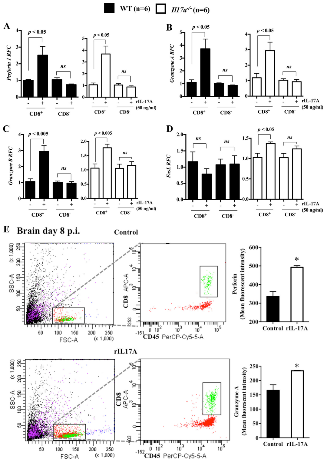
FIG 7 IL-17A induces cytotoxicity mediator gene expression in CD8 + T cells. (A to D) Seven- to 9-week-old WT (C57BL/6J) and Ill17a -/- mice ( n = 6 ) were infected (i.p.) with 100 PFU of WNV and sacrificed at 8 dpi to collect their spleens, followed by magnetic separation of CD8 + T cells. (A to D) RFC of transcripts of perforin-1 (A), granzyme A (B), granzyme B (C), and FasL (D) was measured by qPCR in CD8 + or CD8 - T cells cultured ex vivo for 24 h with or without recombinant mouse IL-17A (50 pg/ml). (E) Eight-week-old Ill17a -/- mice ( n = 4 per group) infected with WNV (100 PFU i.p.) were treated i.p. with recombinant IL-17A (2.5 \mu g/mouse) or PBS (control) at 6 dpi and sacrificed at 8 dpi to characterize brain leukocytes by flow cytometry. The mean fluorescence intensities of perforin and granzyme A within the gated CD45 hi CD8 + cells (green) are shown on the right. All the data (means and SEM) represent the results of two independent experiments compared by two-tailed Student t tests. (A to D) All the data from WT and Ill17a -/- mice were normalized to the respective mock-treated controls. ns , no significant difference ( P > 0.05 ).
