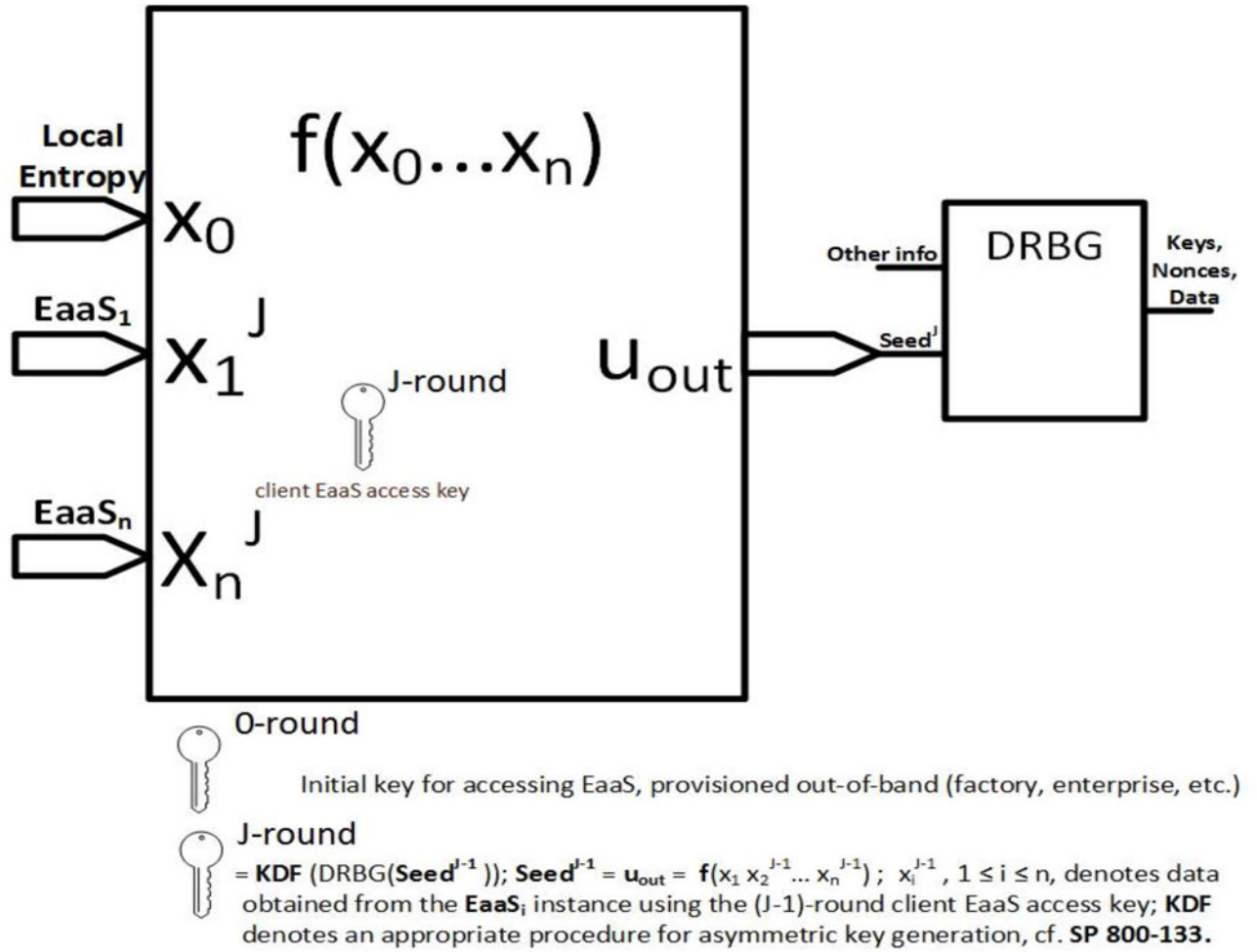
Figure 2. Client key management
