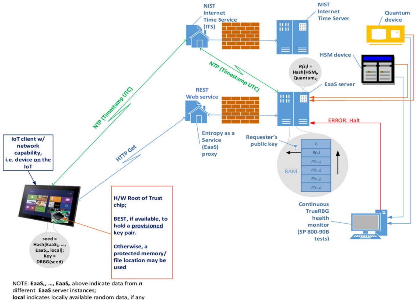
Figure 4. The EaaS Architecture
