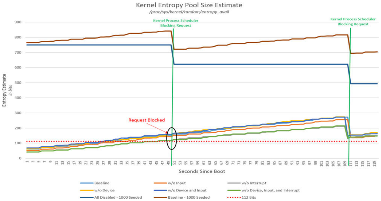
Figure 5. Linux seeded with EaaS
