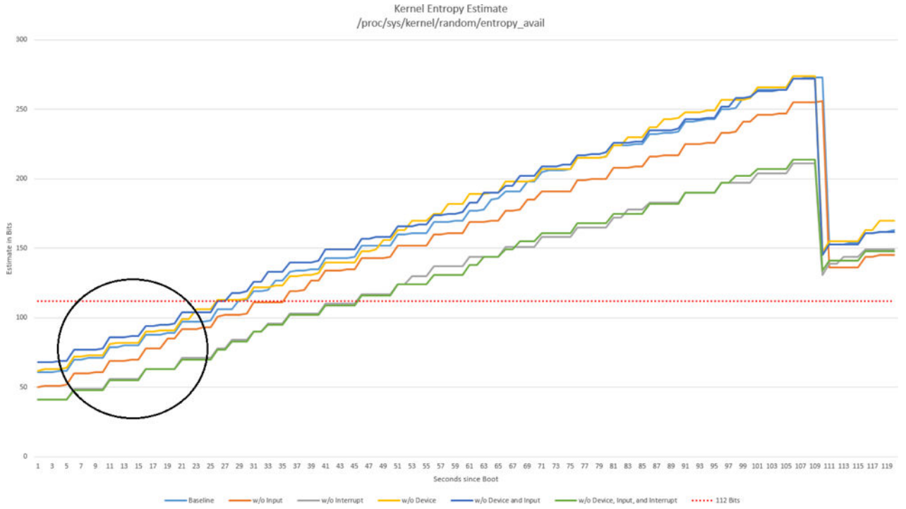
Figure 1. Linux kernel entropy accumulation
