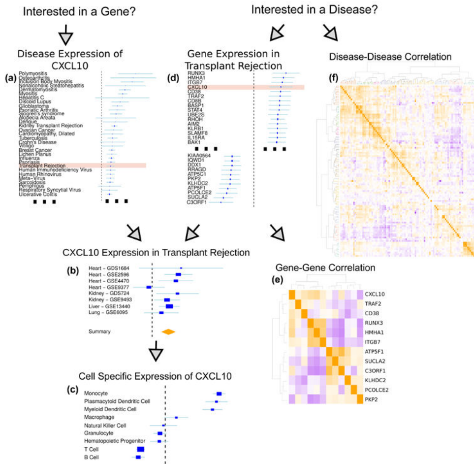
Fig. 2. Diagram of the MetaSignature web application.
