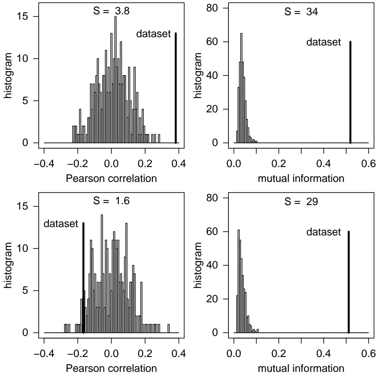
Figure 9 Significance values for the two gene-gene comparisons shown in Figure 8, C and D (top and bottom, respectively) are calculated from 300 shuffled realisations based on the Pearson correlation coefficient (left) and the mutual information (right) as distance measures.
