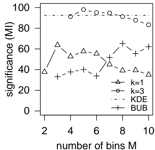
Figure 6 The significance, S , as a function of the number of bins, M , for the two examples of Figure 5, and for the entropy estimator \hat{H}_{BUB} . For kernel density estimators (KDE), the significance, which is not depending on M , is calculated to S = 92 .
