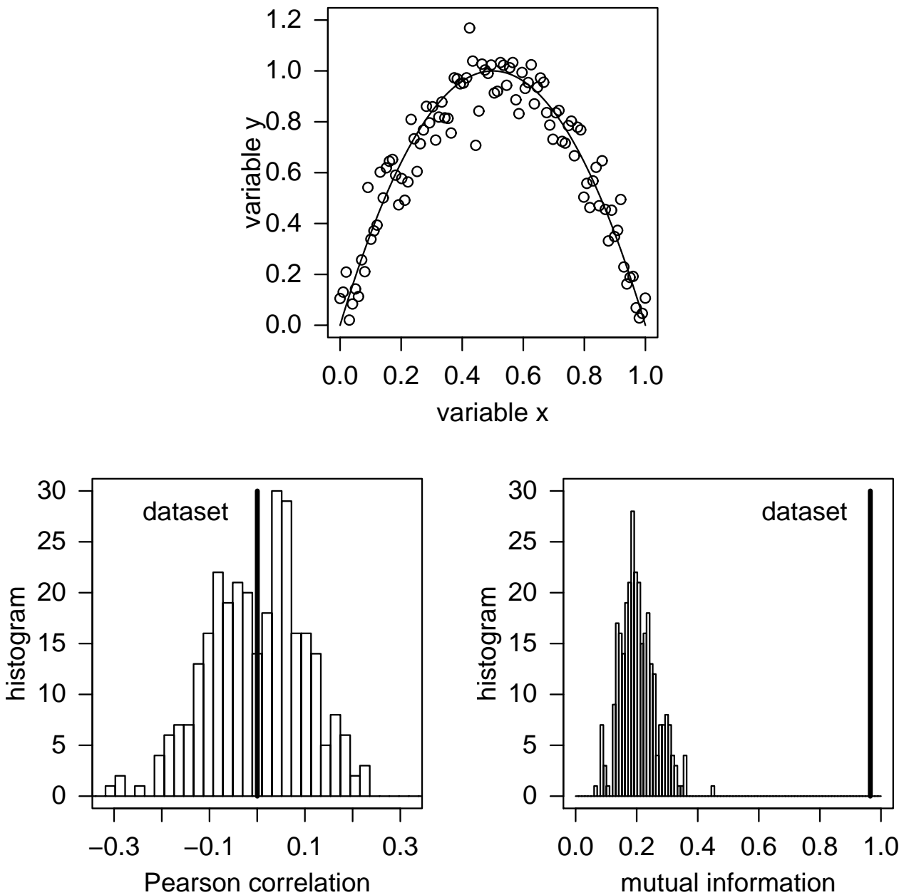
Figure 1 Two datasets X and Y (100 data points) show a hypothetical dependency f(x) = 4x(1 - x) (top). The Pearson correlation coefficient is not able to detect a significant correlation as shown in the histogram plot of the dataset compared to 300 realisations of shuffled data (left). Mutual information clearly shows that the two datasets are not statistically independent (right).
