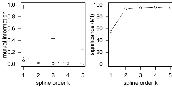
Figure 4 Mutual information calculated for a dataset of 300 data points drawn from the distribution shown in Figure 1 (crosses). The number of bins was fixed to M = 6 . The average mutual information for 300 shuffled realisations of the dataset is shown (circles) together with the standard deviation as error-bars. The largest value found within the ensemble of shuffled data is drawn as a dotted line (left). The significance was calculated from Eq. (13) (right).
