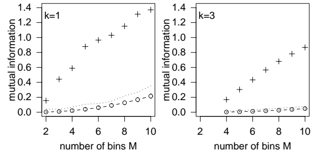
Figure 5 Based on the distribution of Figure 1, the mutual information for 300 data points and two spline orders k = 1 and k = 3 is shown as a function of the number of bins M (crosses) together with mean (circles) and standard deviations (error-bars) of 300 surrogates. The dotted lines indicate the largest mutual information found within the ensemble of surrogate data.
