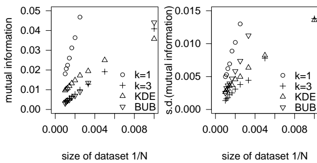
Figure 3 Mutual information is estimated for artificially generated equidis-tributed random numbers from the simple binning ( k = 1 ), the B-spline approach ( k = 3 ), and the entropy estimator \hat{H}_{BUB} using M = 6 bins, and additionally from the kernel density estimator. The average over an ensemble of 600 trials is shown as a function of the size of the dataset (left) together with the standard deviation (right).
