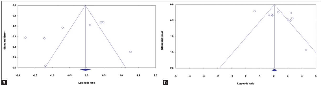
Figure 2: Begg's funnel plot of the meta-analysis of prostate cancer risk and p53 codon 72 polymorphism. (a) Allelic model: C versus G, and (b) dominant model: CC + CG versus GG
