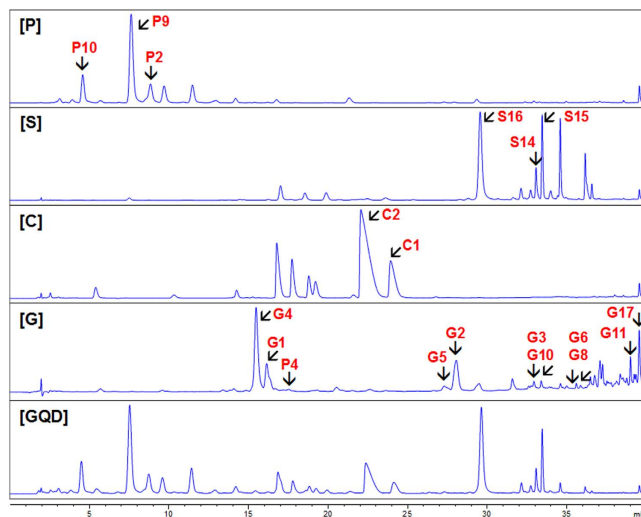
Figure 2. HPLC fingerprints of GQD and its component herbs, showing the single compounds selected for metabolic studies. P, Puerariae Lobatae Radix; S, Scutellariae Radix; C, Coptidis Rhizoma; G, Glycyrrhizae Radix et Rhizoma Praeparata cum Melle. UV wavelength of P, S, C, G and GQD were 254 nm, 270 nm, 270 nm, 300 nm, and 270 nm, respectively. Black arrows show representative compounds.
